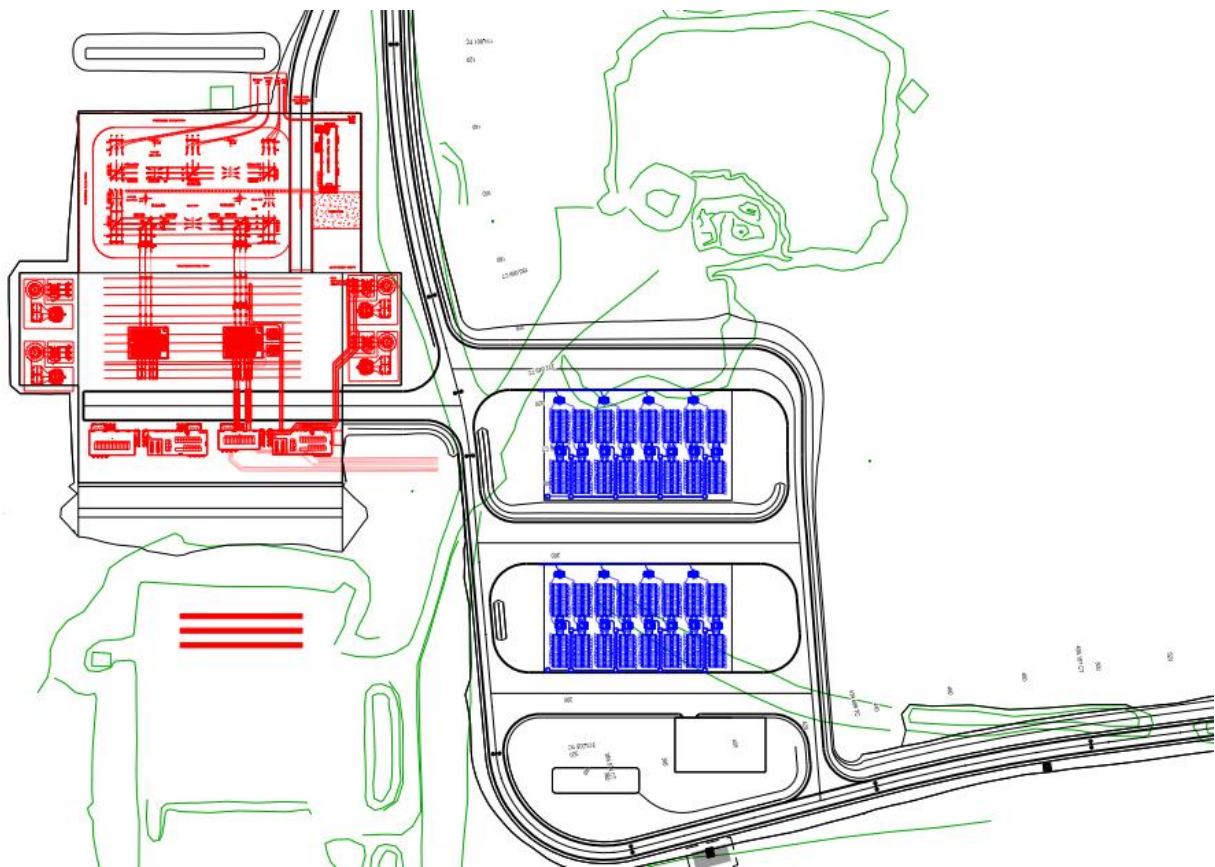
Figure 2 Springvale Hub Site layout - WiP_Site_Layout_01_ WiP Site Layout Rev.A
