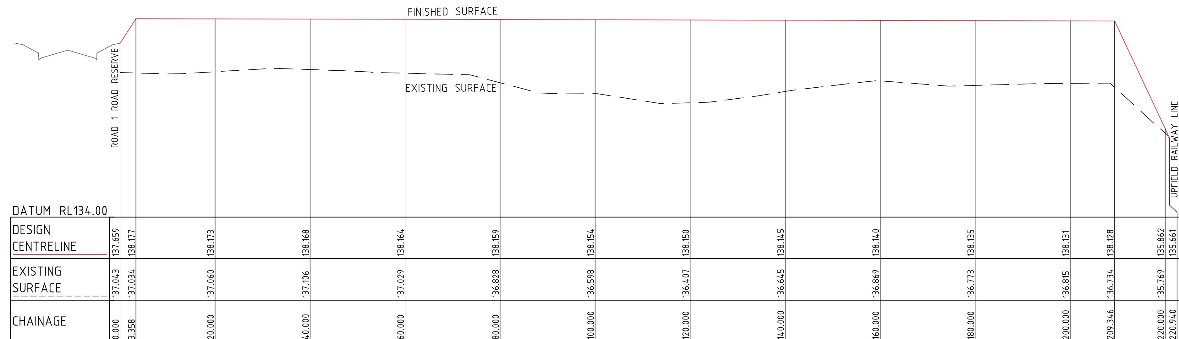
SECTION C-C
