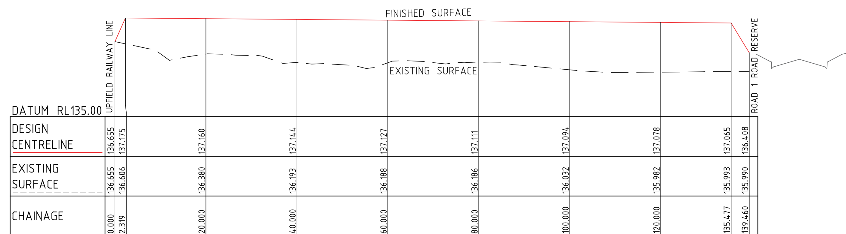
SECTION E-E
