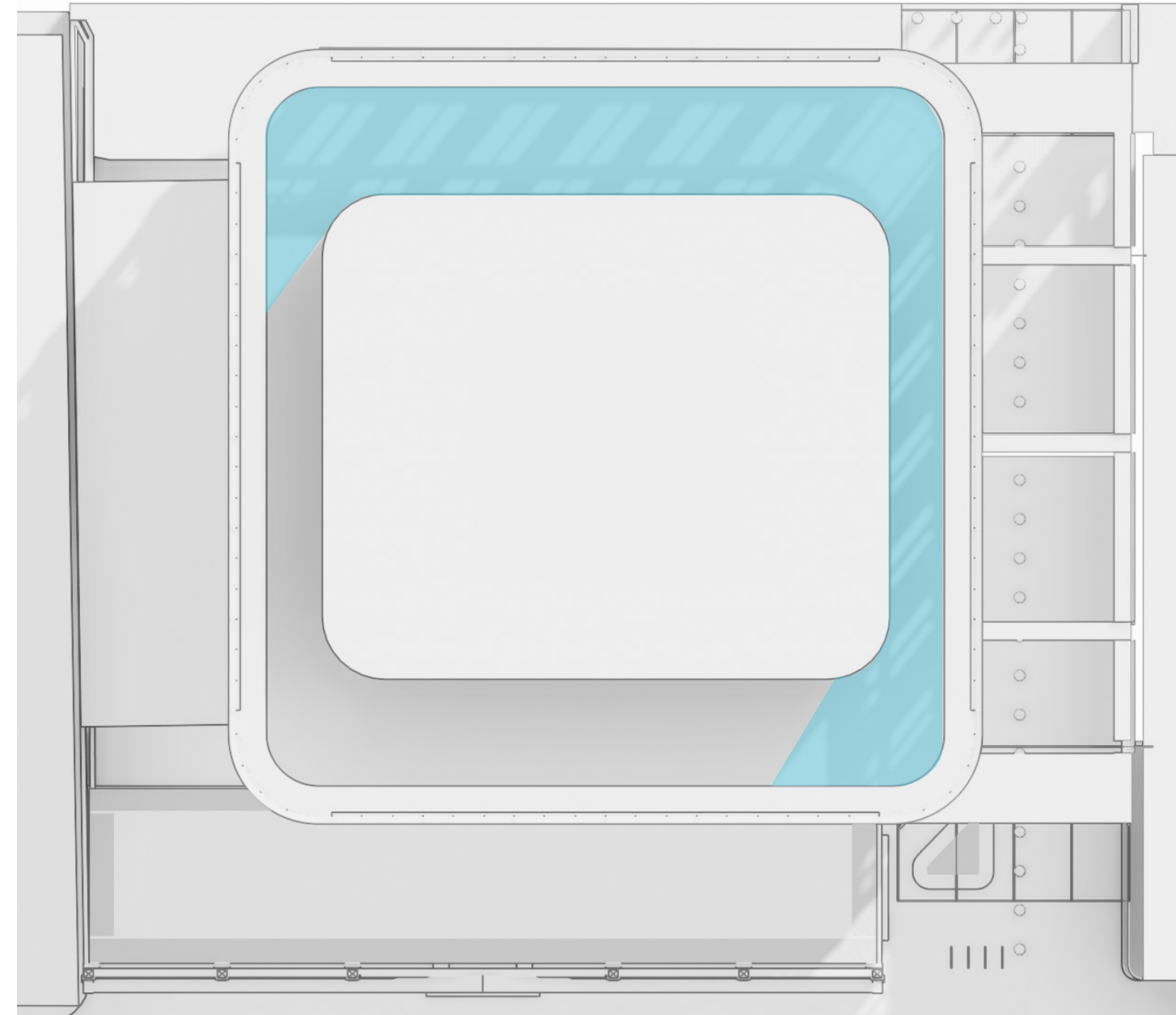
June 21 - 13:00 ROOFTOP TERRACE AREA: 435M2 ROOFTOP TERRACE AREA IN SUNLIGHT: 196M2 (45%)
