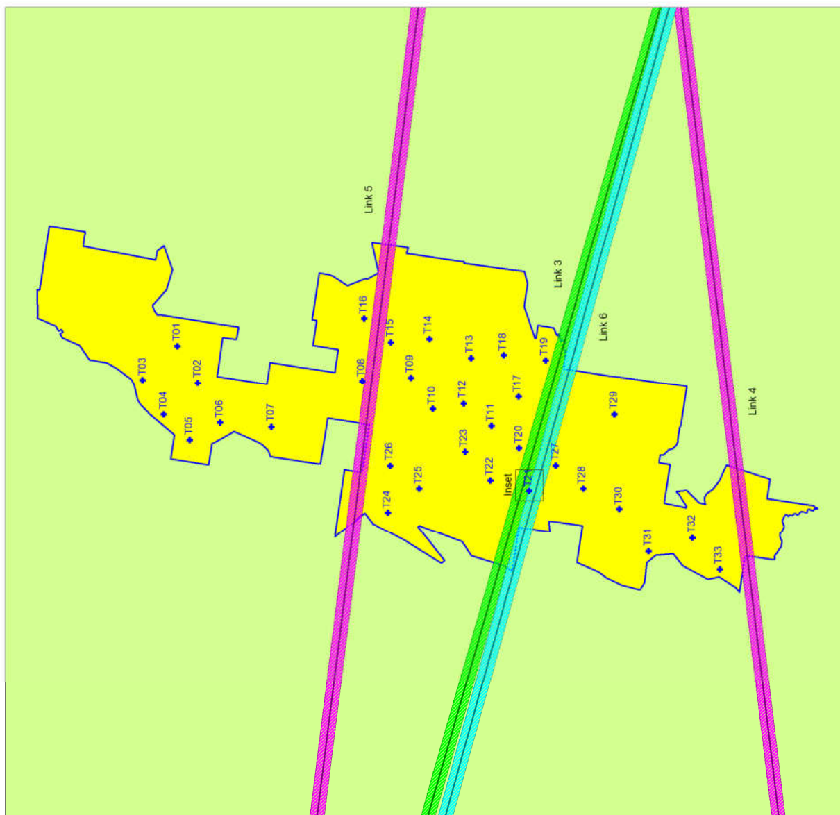
Figure 6 Identified point-to-point radiocommunication vectors operated by Digital Distribution Australia, Optus Mobile, and VerTel and requested clearance zones for the proposed Project
