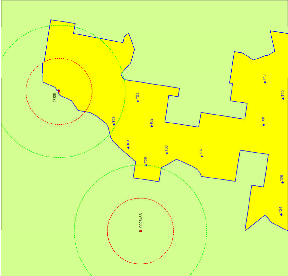
Figure 3 Identified radiocommunication sites within 2 km of the turbine locations for the proposed Project
