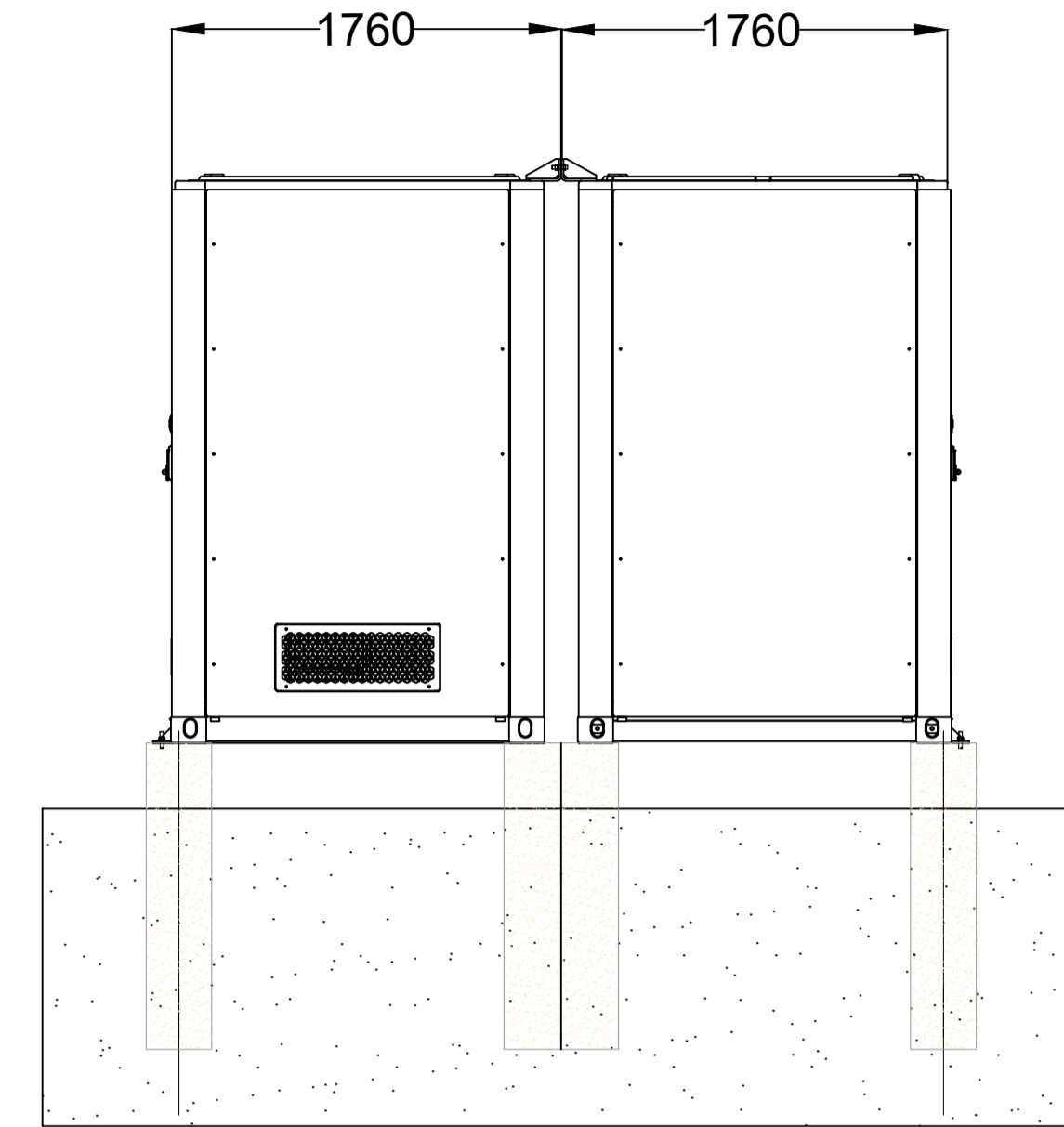
SIDE VIEW
