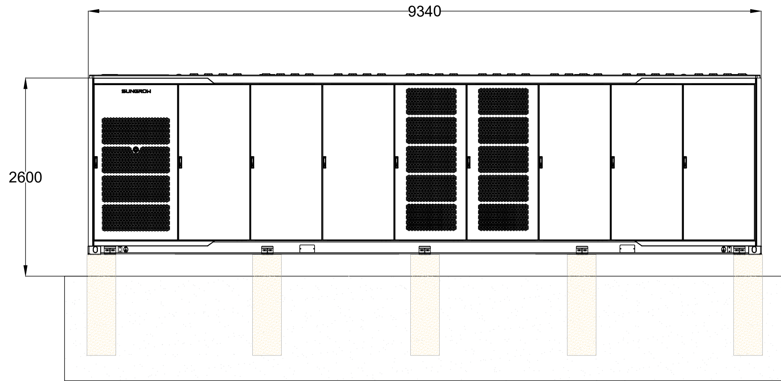
FRONT VIEW
