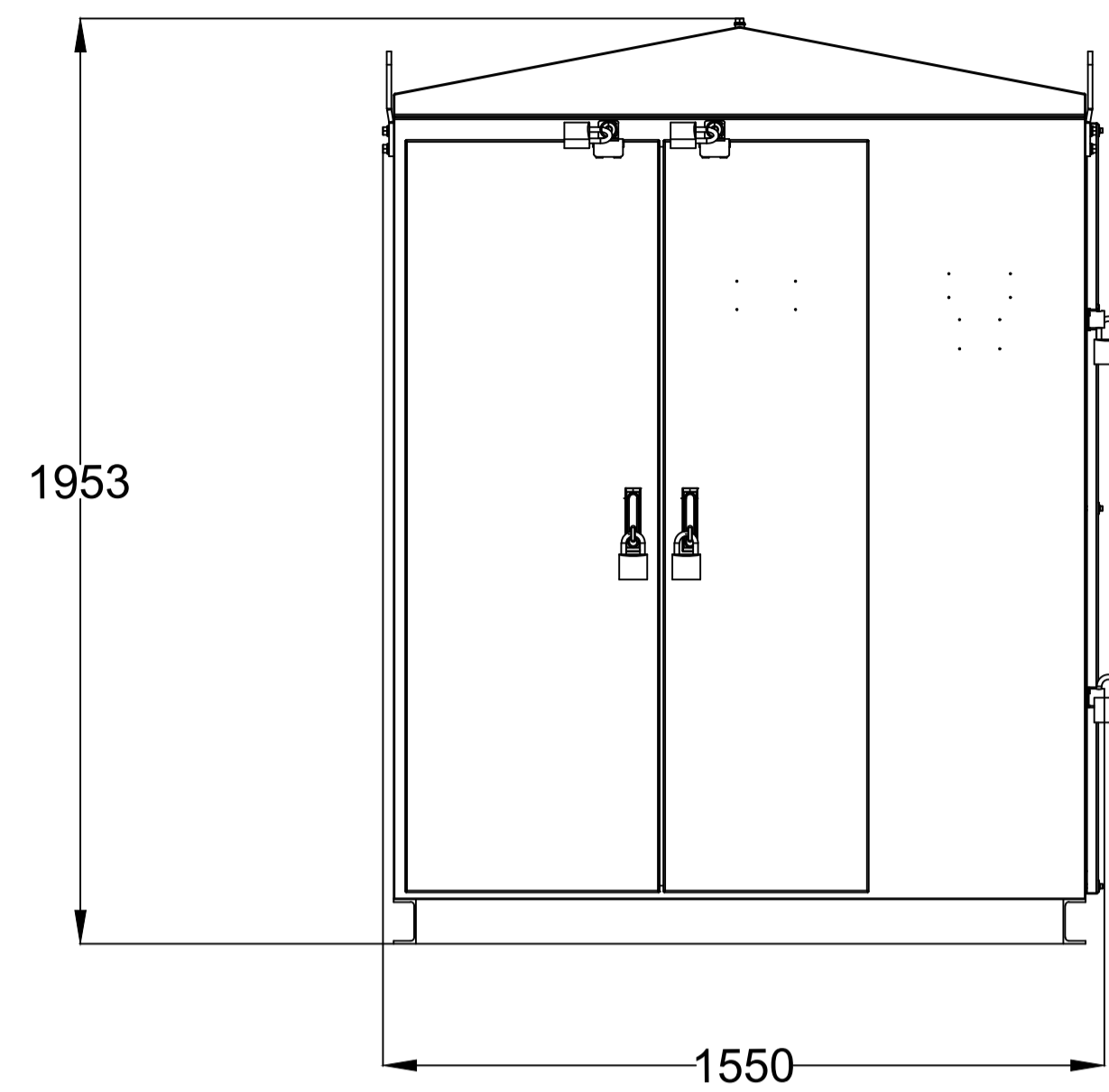
FRONT VIEW
