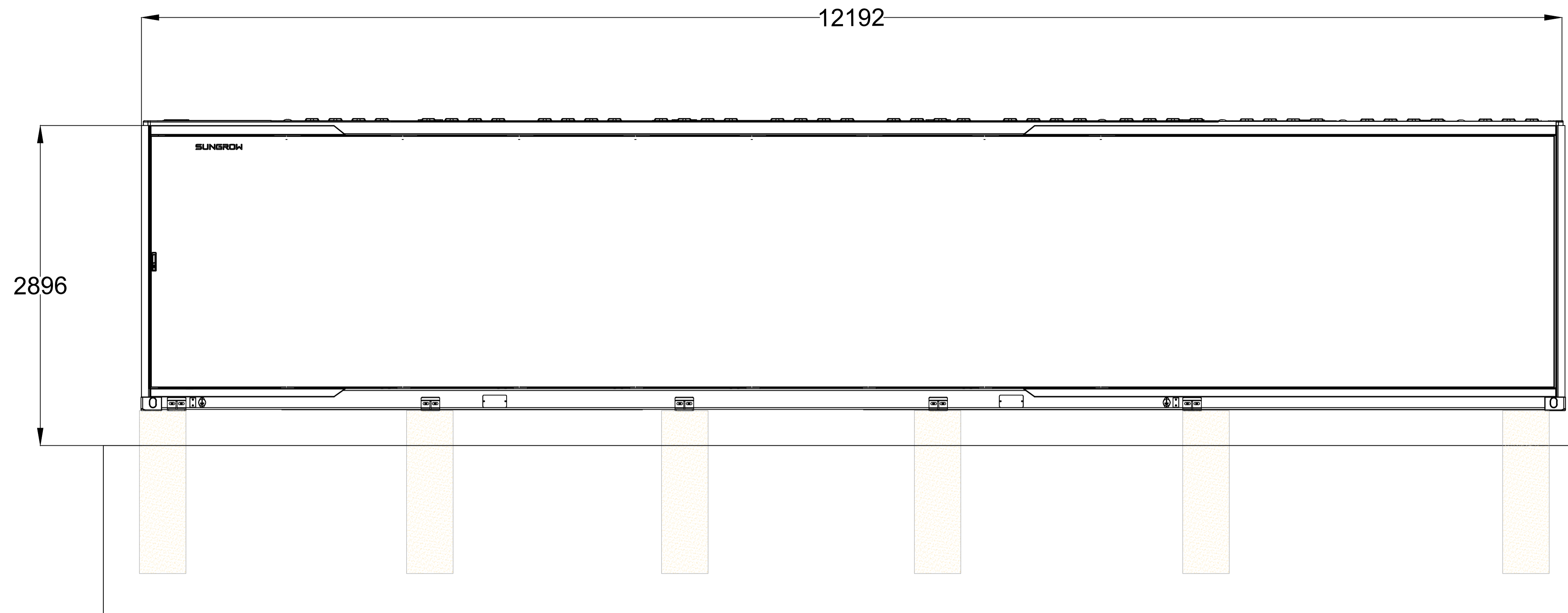
FRONT VIEW
