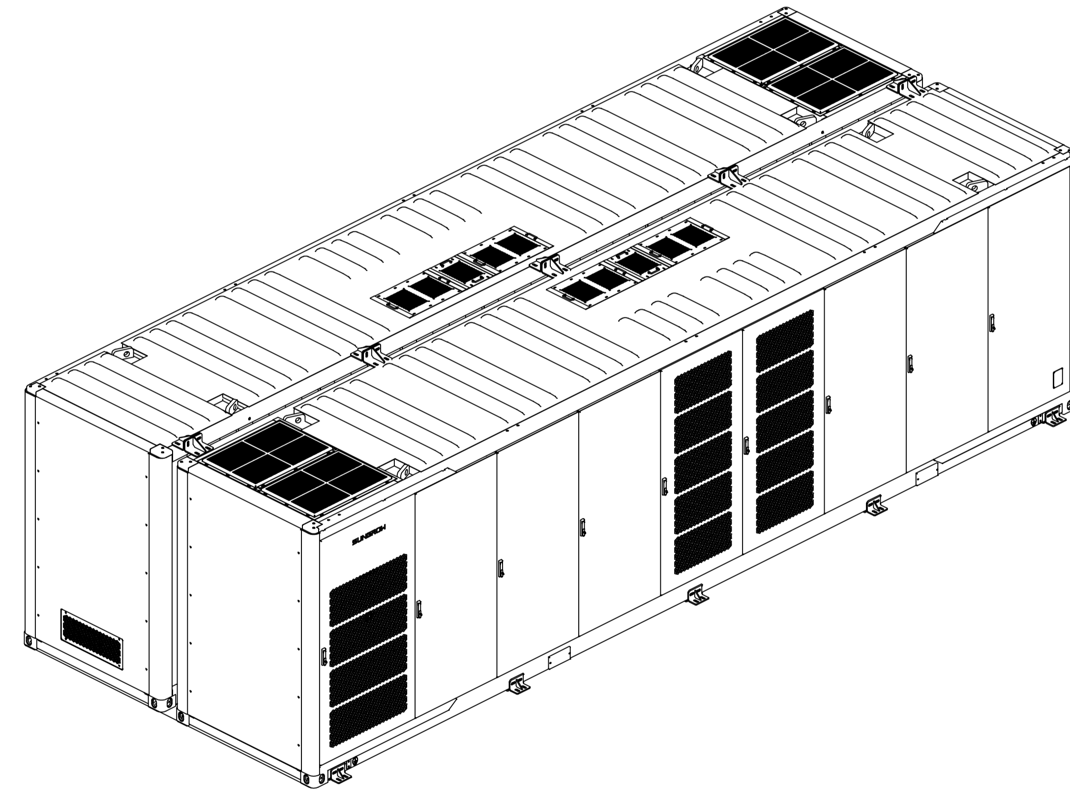
ISOMETRIC VIEW - 2 CONTAINERS
