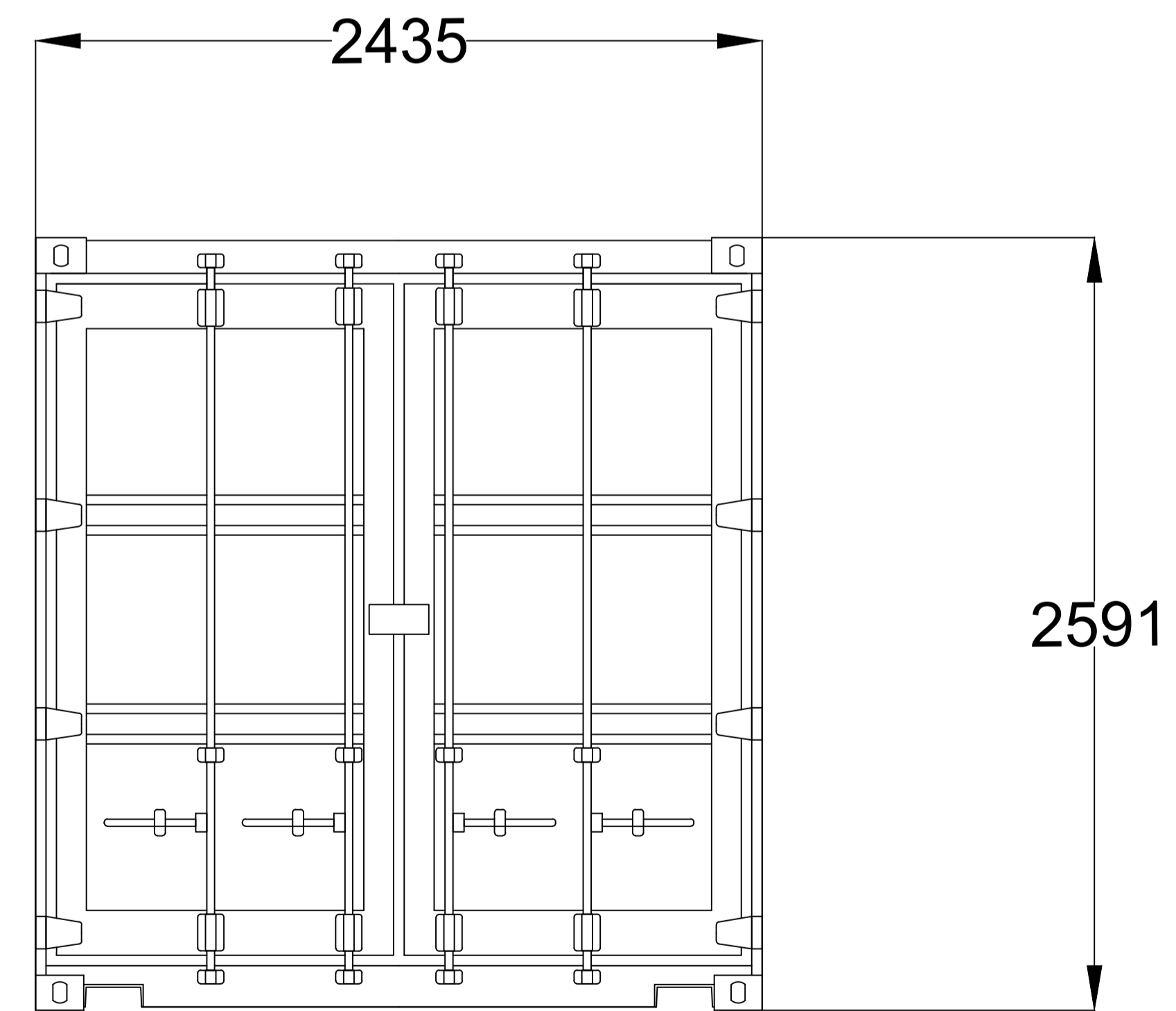
SIDE VIEW
