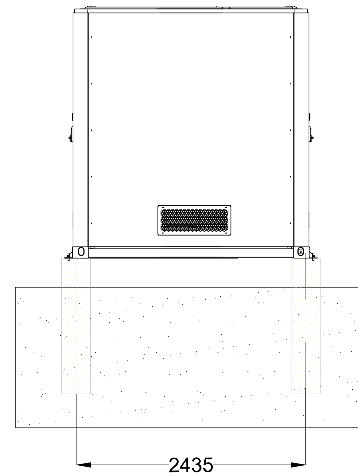
SIDE VIEW
