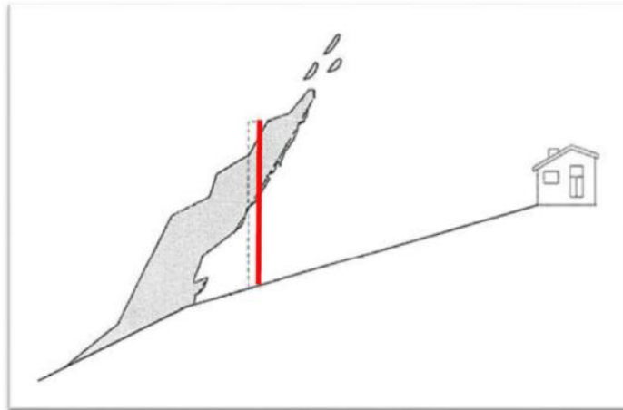
Figure 1 – Standard 'view factor' scenario in AS3959 (Red line indicates emitter and house indicates the site)
