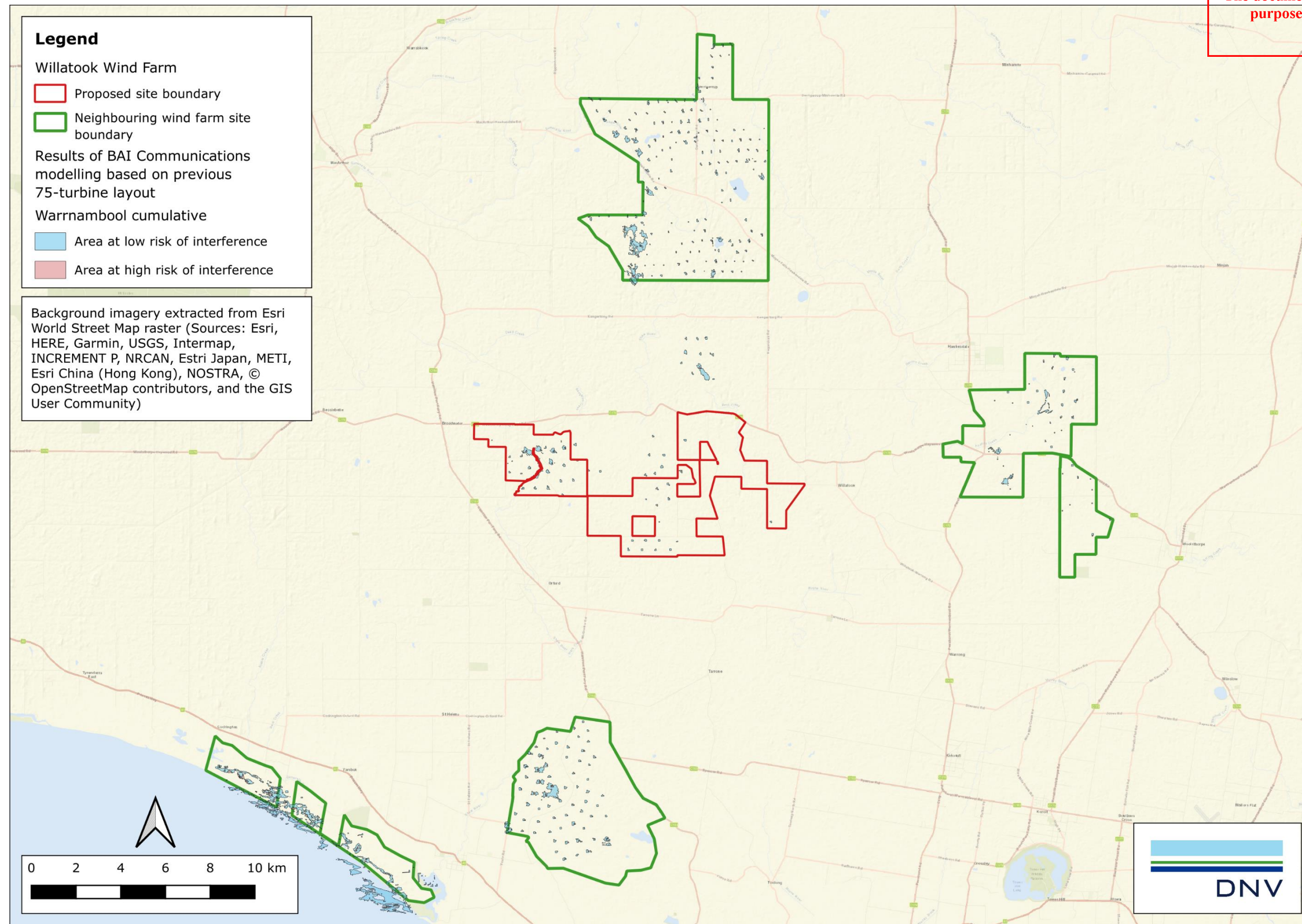
Figure 22 Potential television EMI zones for the Warrnambool (Tower Hill) broadcast tower from the proposed Project in conjunction with neighbouring wind farm developments, considering the availability of alternative signals from other towers
