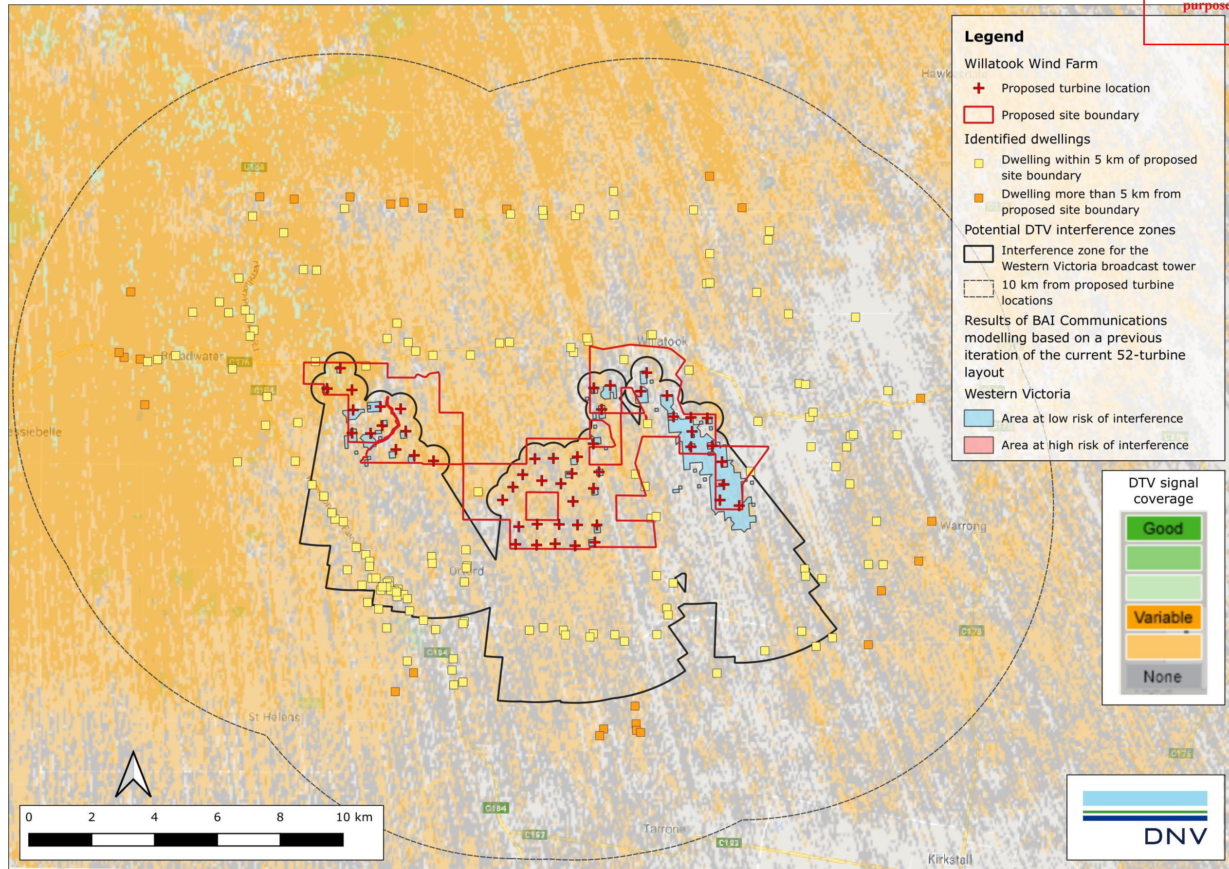
Figure 20 Potential television EMI zones for the Western Victoria (Mt Dundas) broadcast tower from the proposed Project
