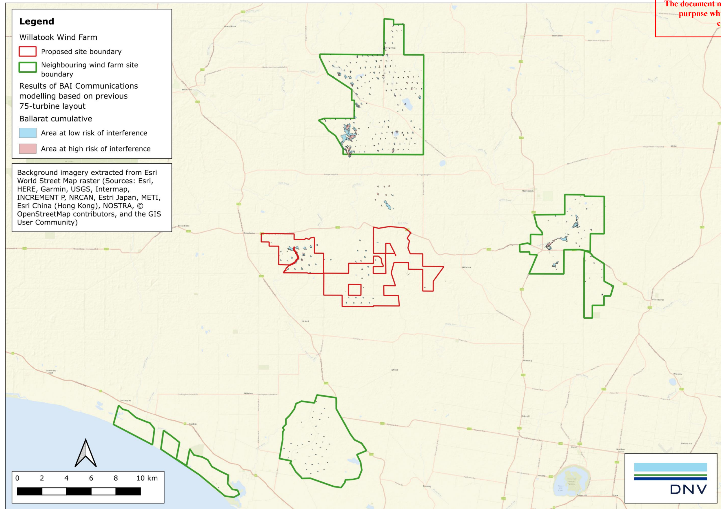
Figure 25 Potential television EMI zones for the Ballarat (Lookout Hill) broadcast tower from the proposed Project in conjunction with neighbouring wind farm developments, considering the availability of alternative signals from other towers
