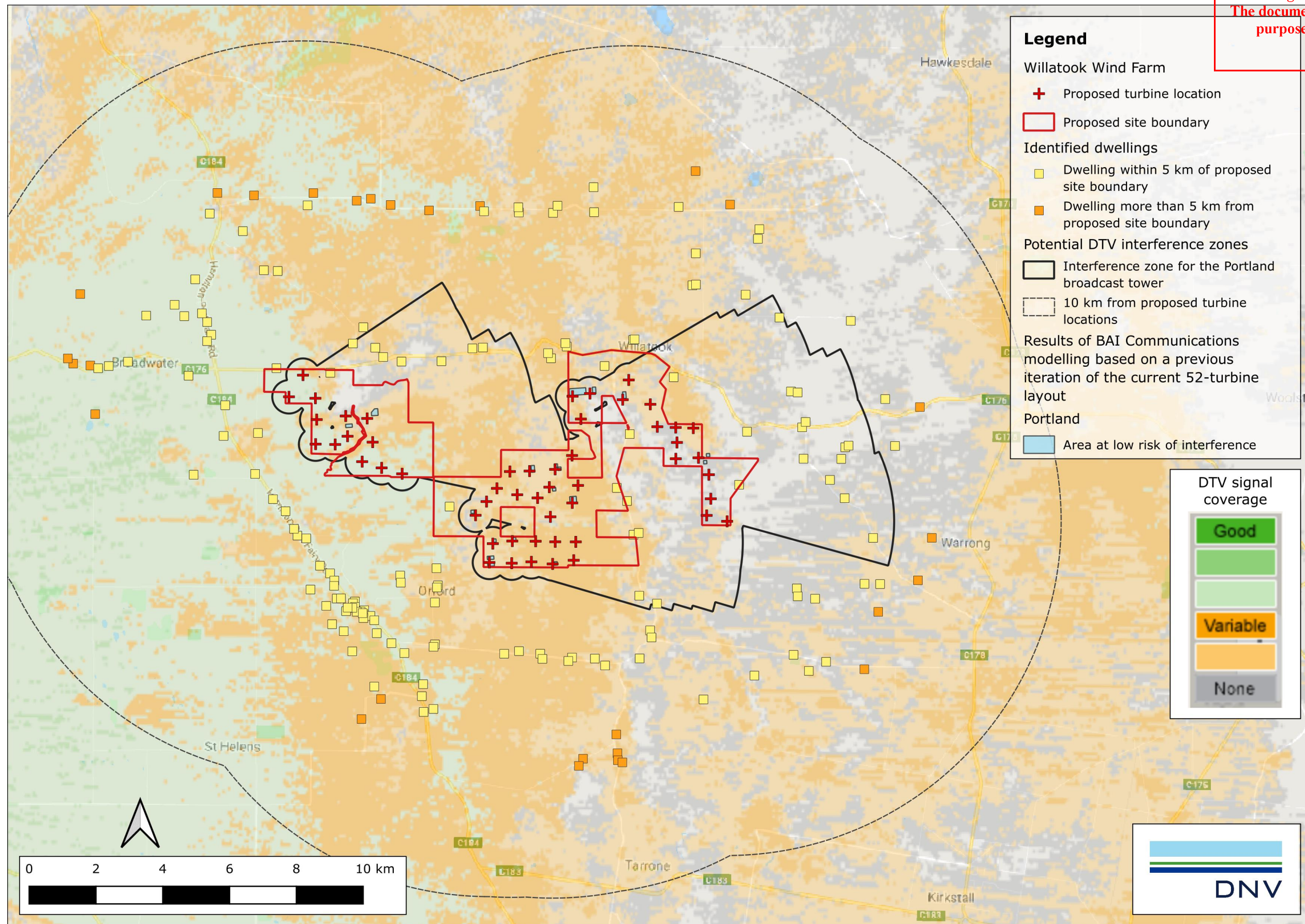
Figure 19 Potential television EMI zones for the Portland (Narrawong/Mt Clay) broadcast tower from the proposed Project
