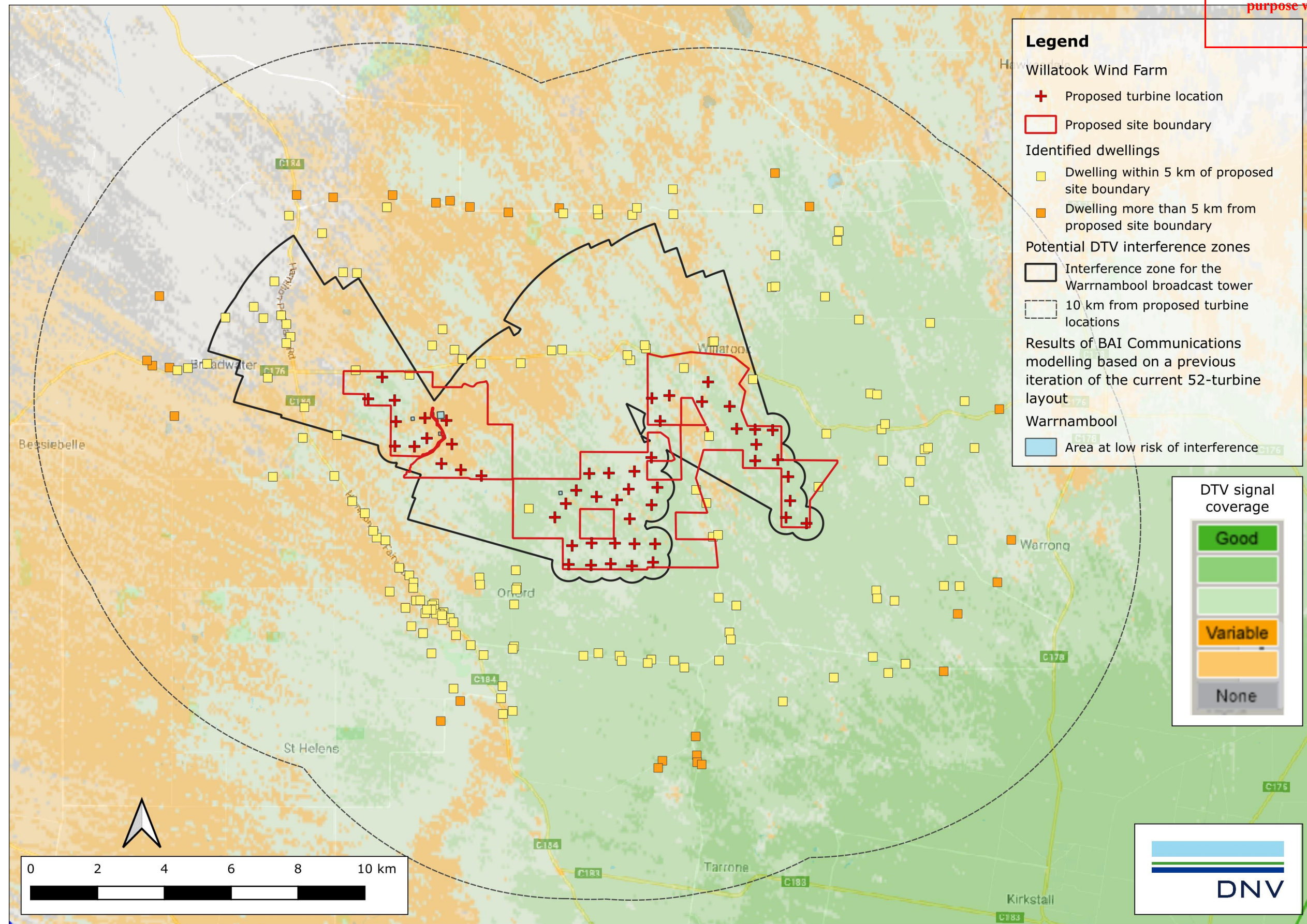
Figure 18 Potential television EMI zones for the Warrnambool (Tower Hill) broadcast tower from the proposed Project
