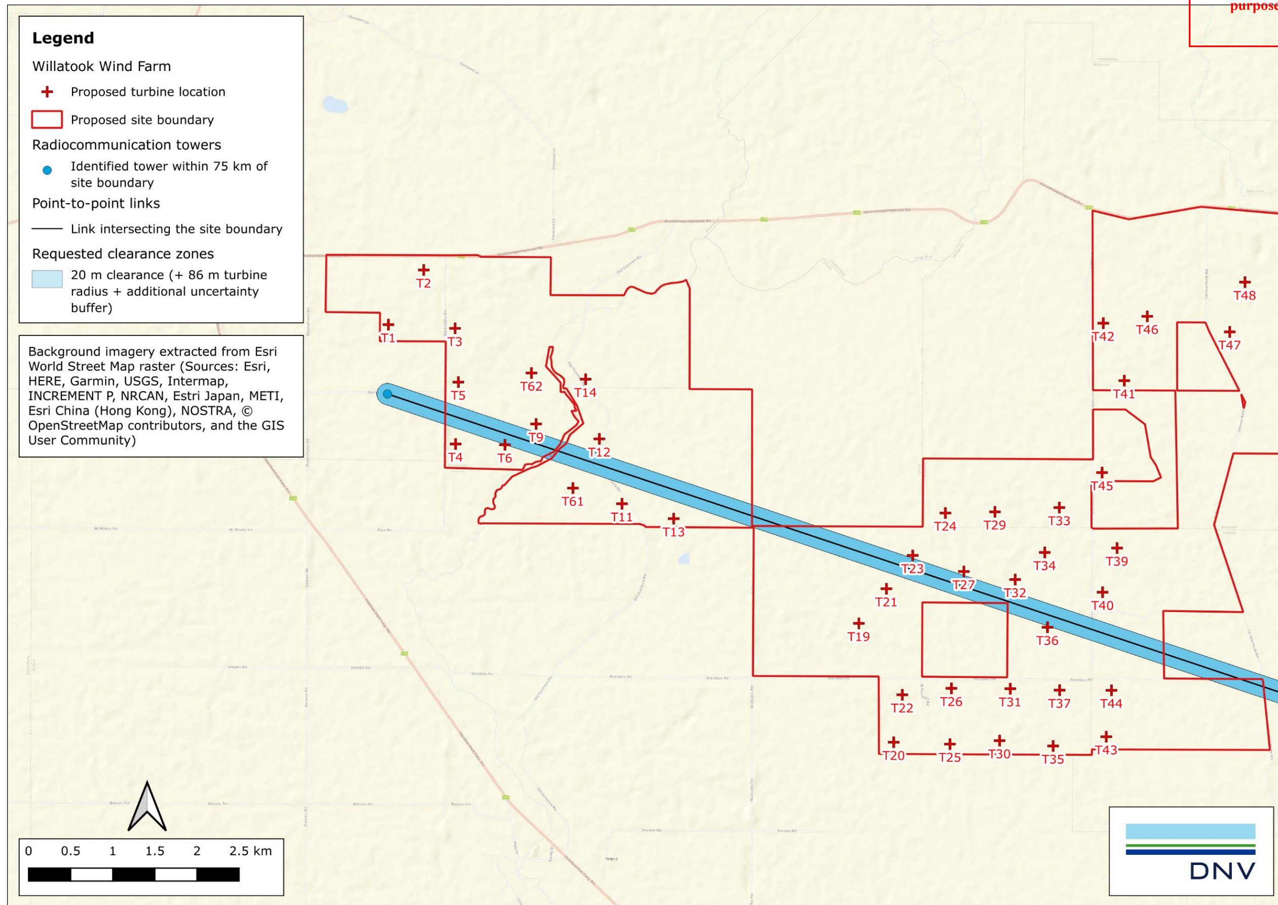
Figure 6 Identified point-to-point radiocommunication vectors and requested clearance zones by AusNet Services
