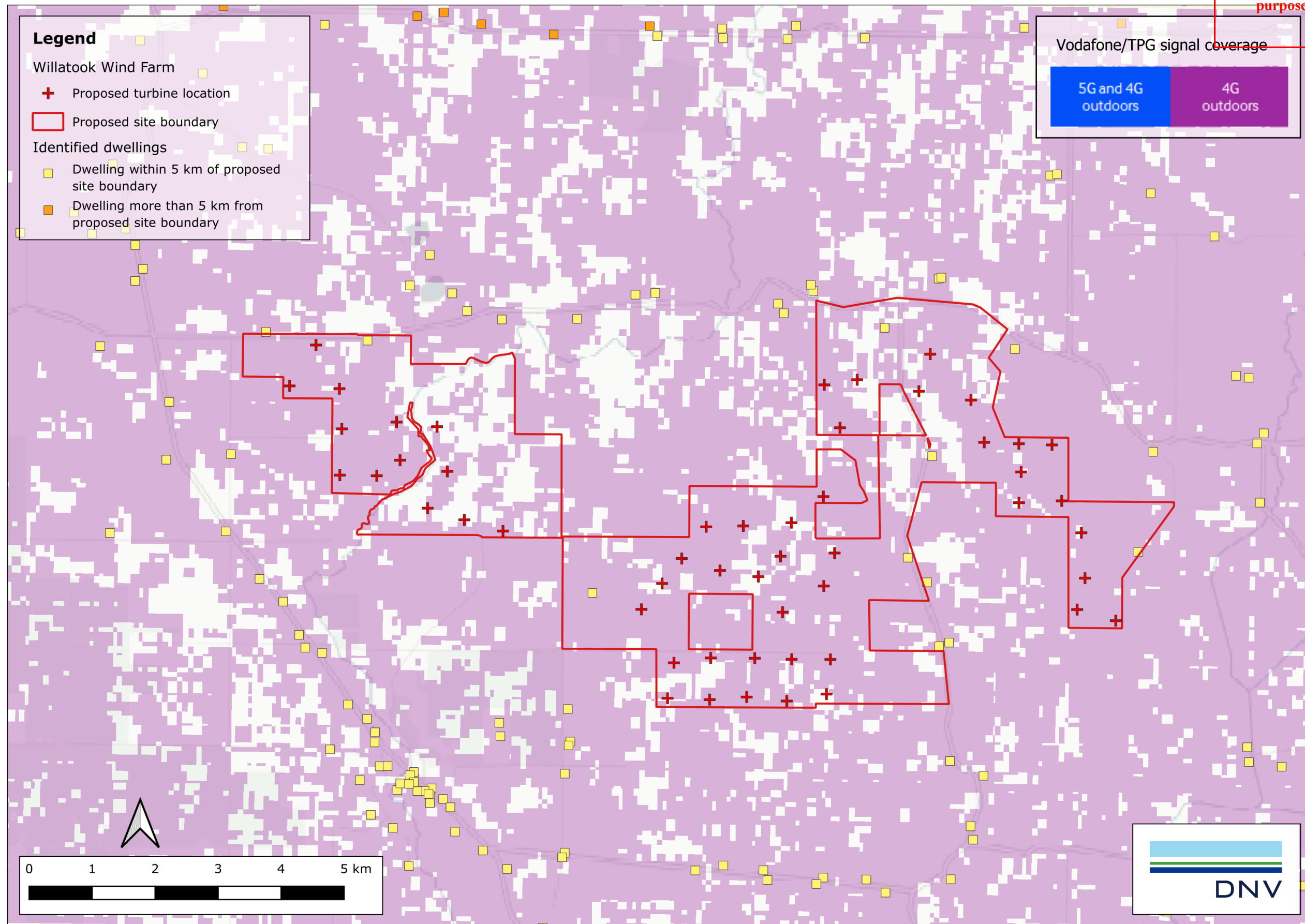
Figure 15 Vodafone/TPG network coverage (Apple iPhone 13 handset) for the proposed Project
