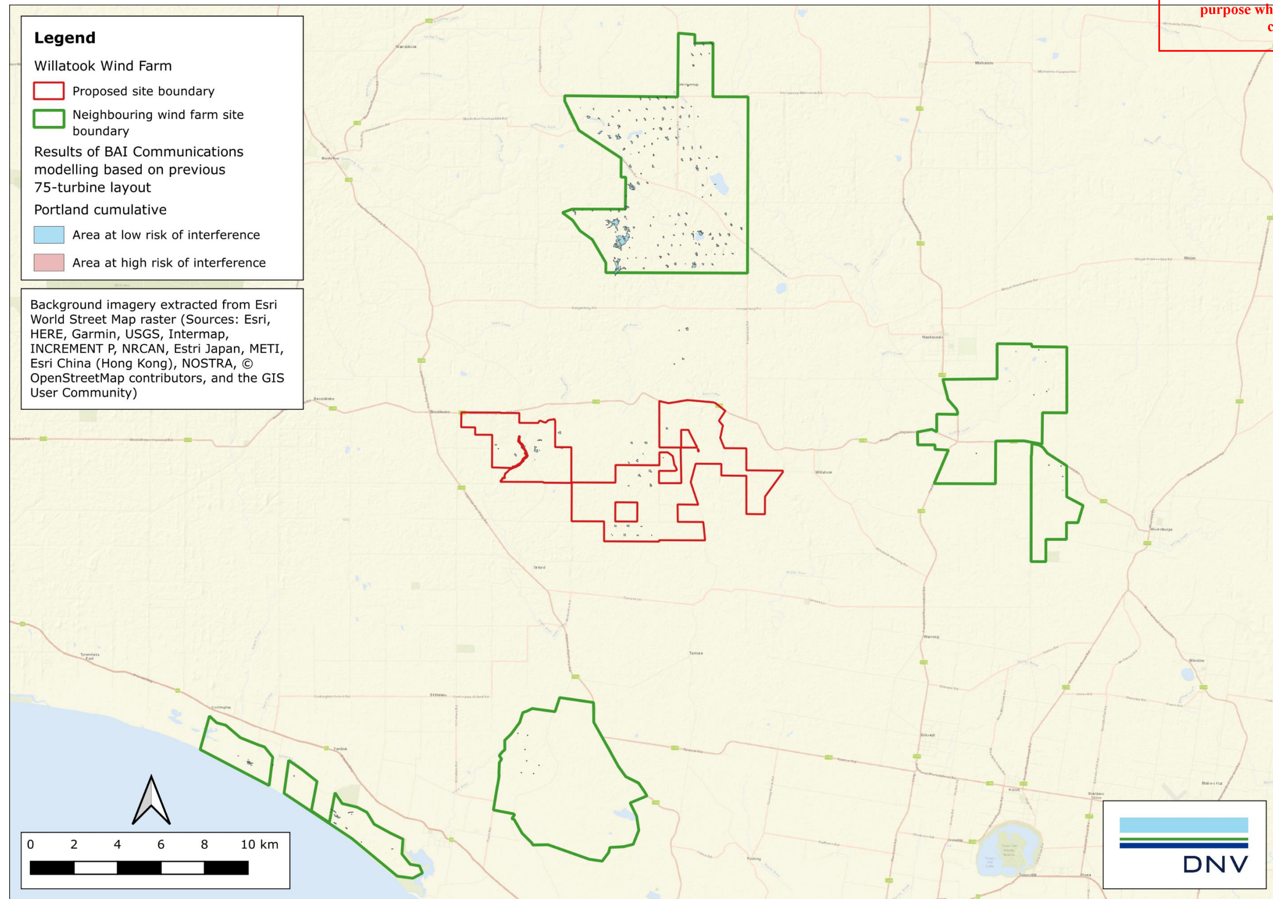
Figure 23 Potential television EMI zones for the Portland (Narrawong / Mt Clay) broadcast tower from the proposed Project in conjunction with neighbouring wind farm developments, considering the availability of alternative signals from other towers
