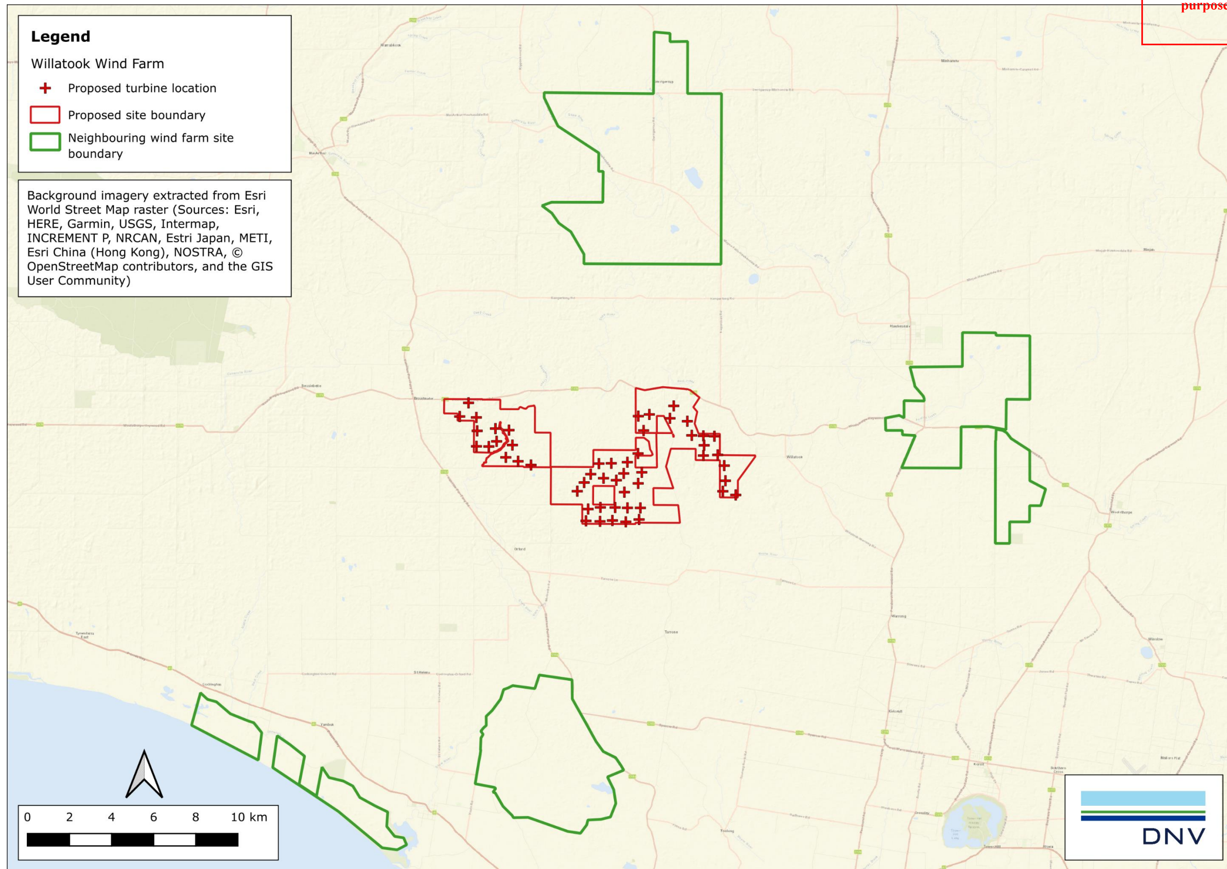
Figure 21 Map of the proposed Project, showing neighbouring wind farm developments
