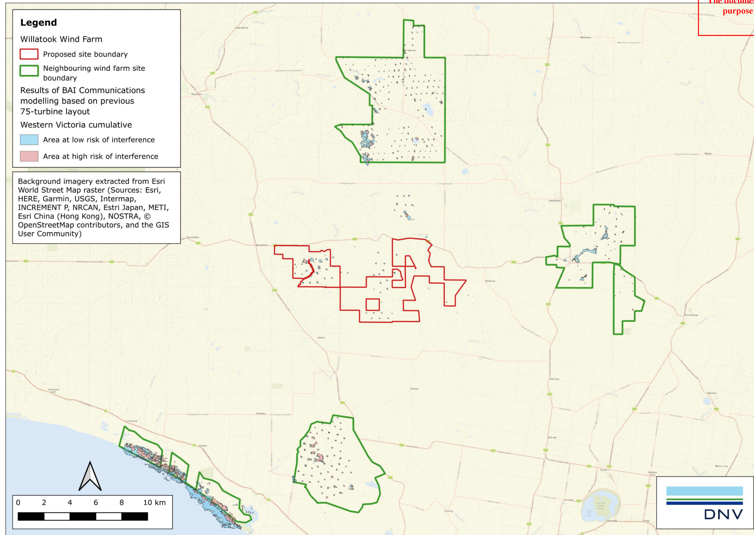
Figure 24 Potential television EMI zones for the Western Victoria (Mt Dundas) broadcast tower from the proposed Project in conjunction with neighbouring wind farm developments, considering the availability of alternative signals from other towers
