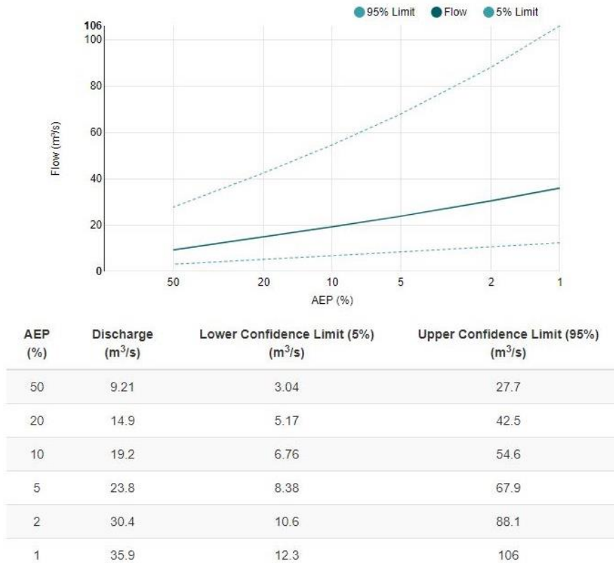
FIGURE 19 DISCHARGES FOR DIFFERENT ANNUAL EXCEEDANCE PROBABILITIES
