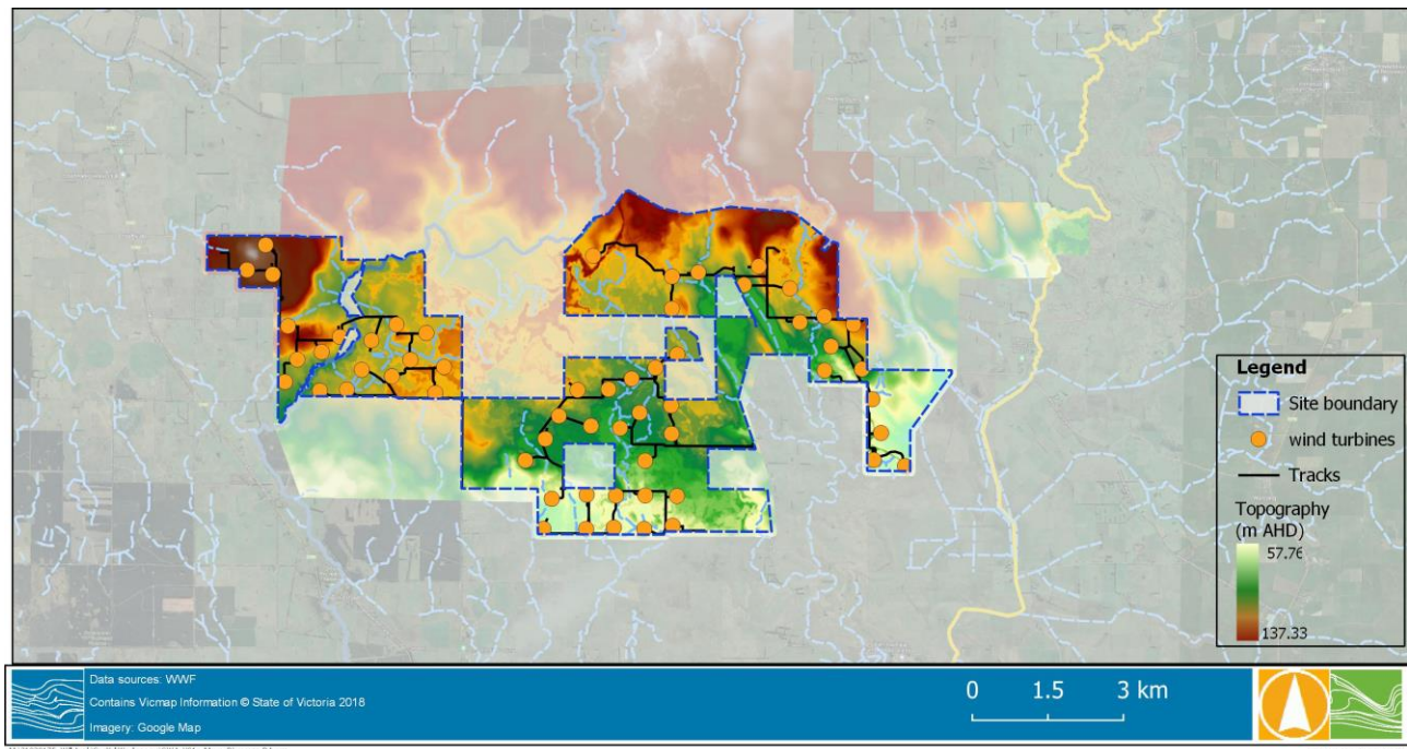
FIGURE 14 LIDAR DATA COVERING THE WWF DEVELOPMENT SITE
