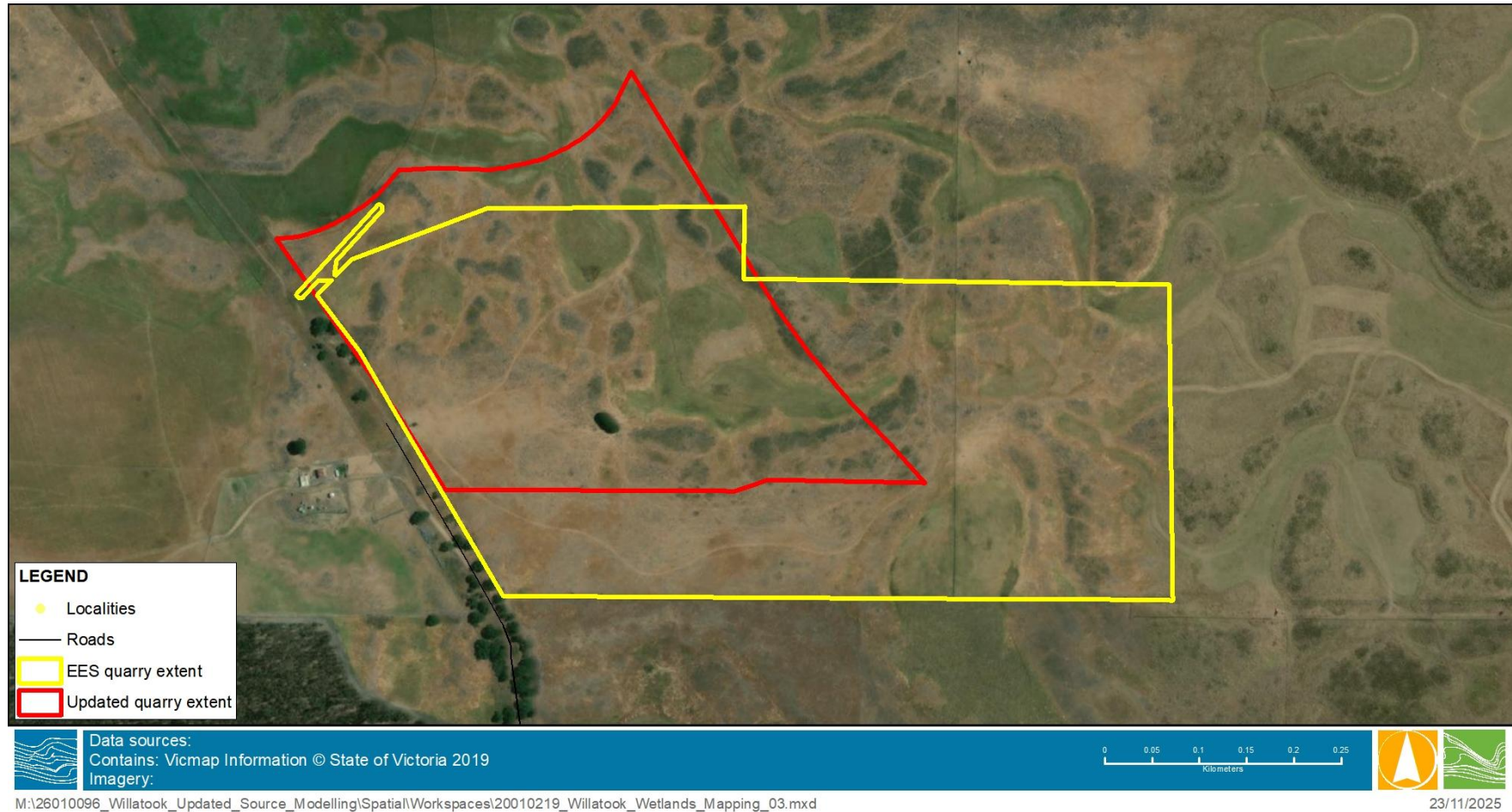
Figure A-4 Wind farm quarry extent changes
