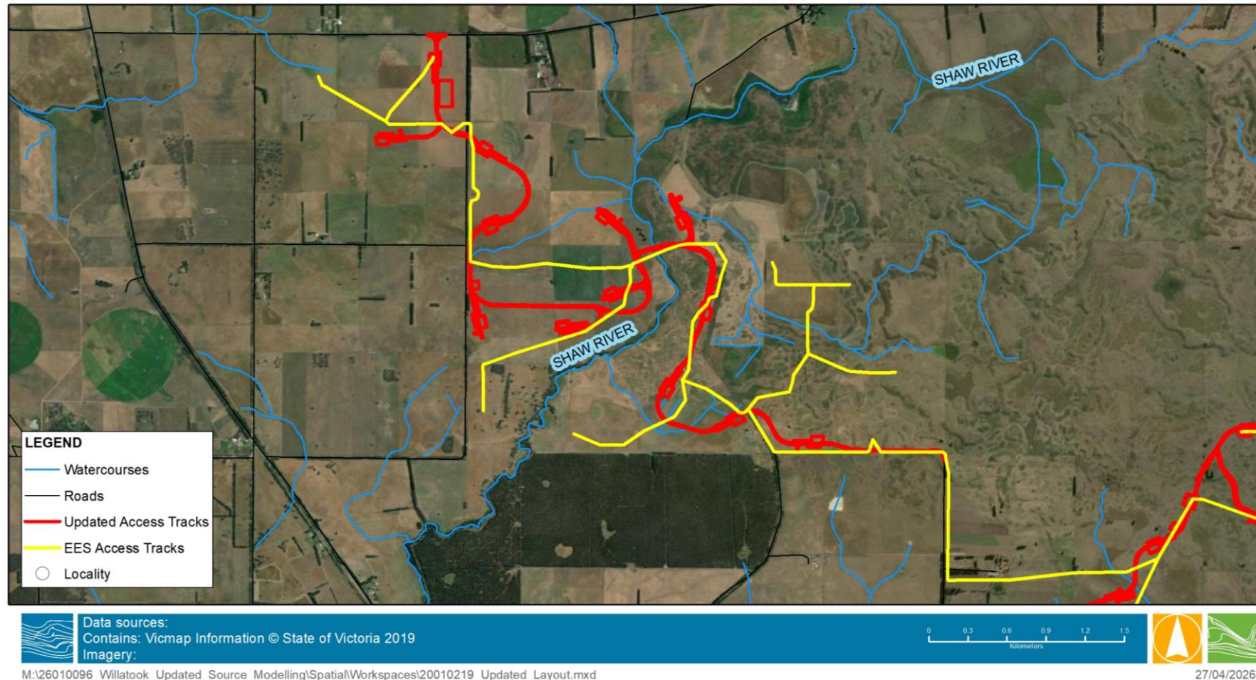
Figure 3-2 Area 1 – access track waterway crossings
