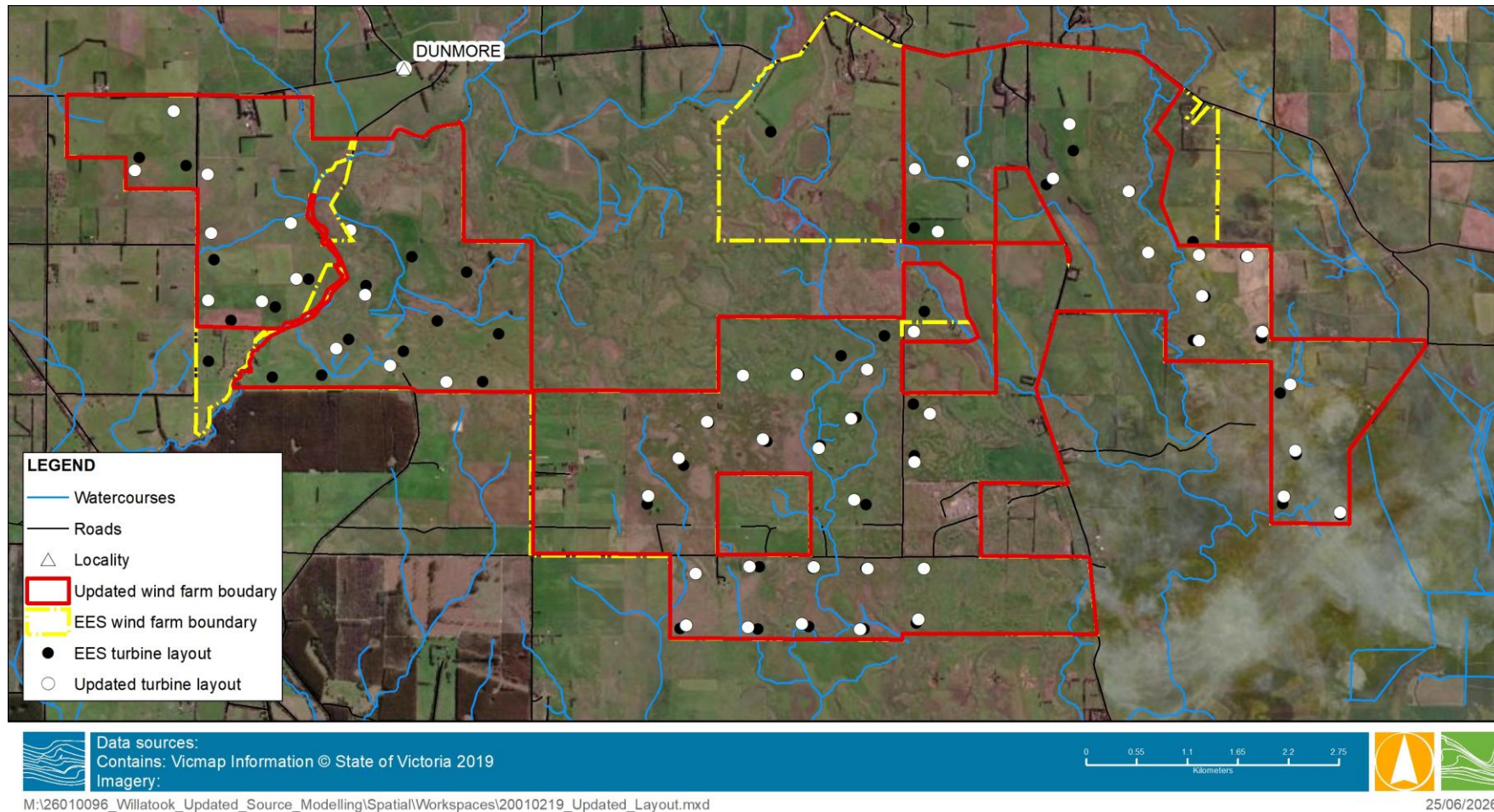
Figure A-1 Wind farm turbine layout and boundary changes
