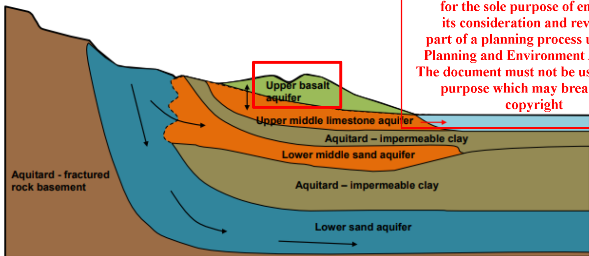
FIGURE 32 REGIONAL CONCEPTUAL MODEL WITH INDICATION OF PROJECT LOCATION HIGHLIGHTED (SOURCE: SOUTH WEST VICTORIA GROUNDWATER ATLAS SRW, 2011)
