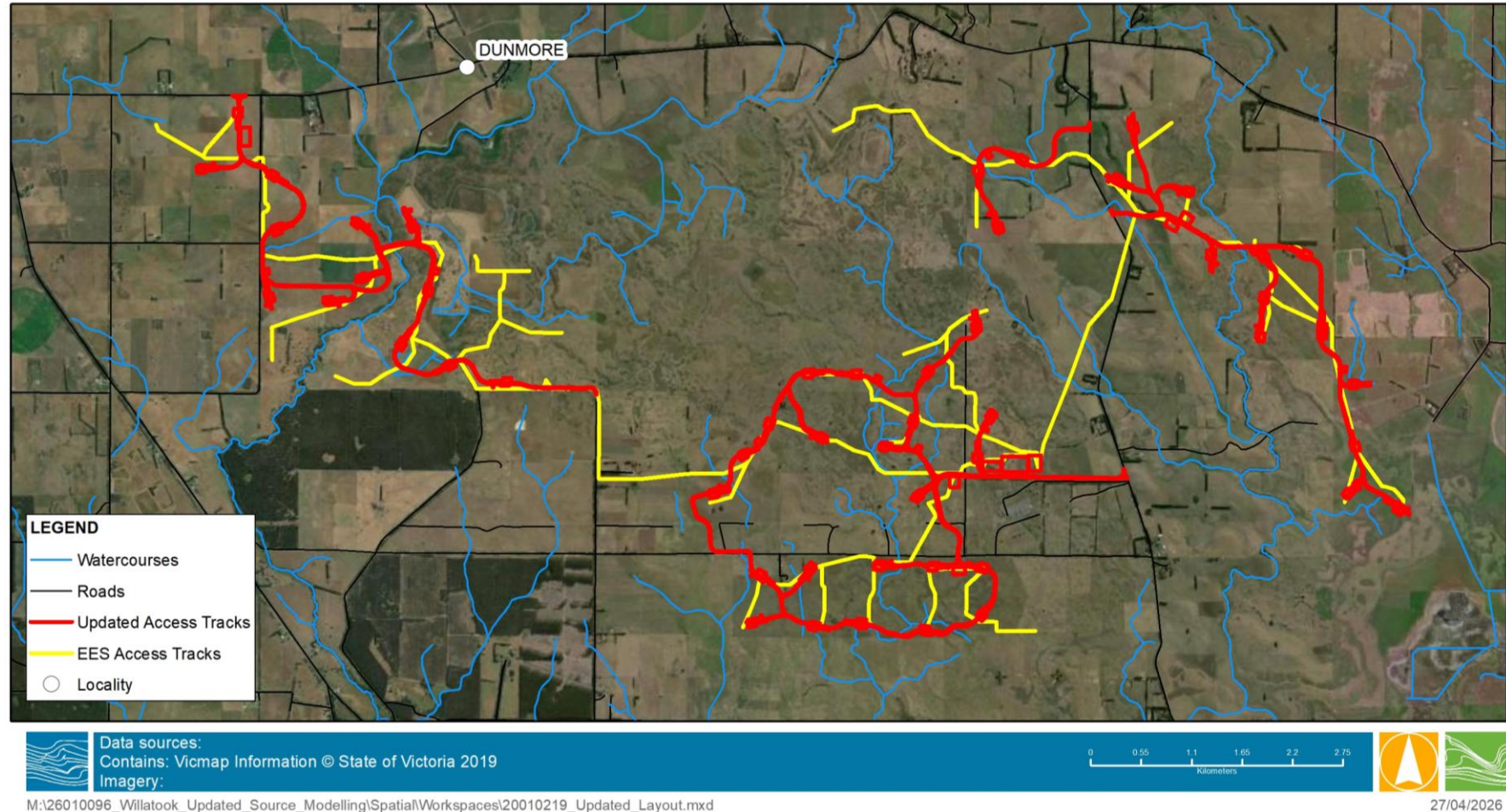
Figure A-2 Wind farm internal track changes
