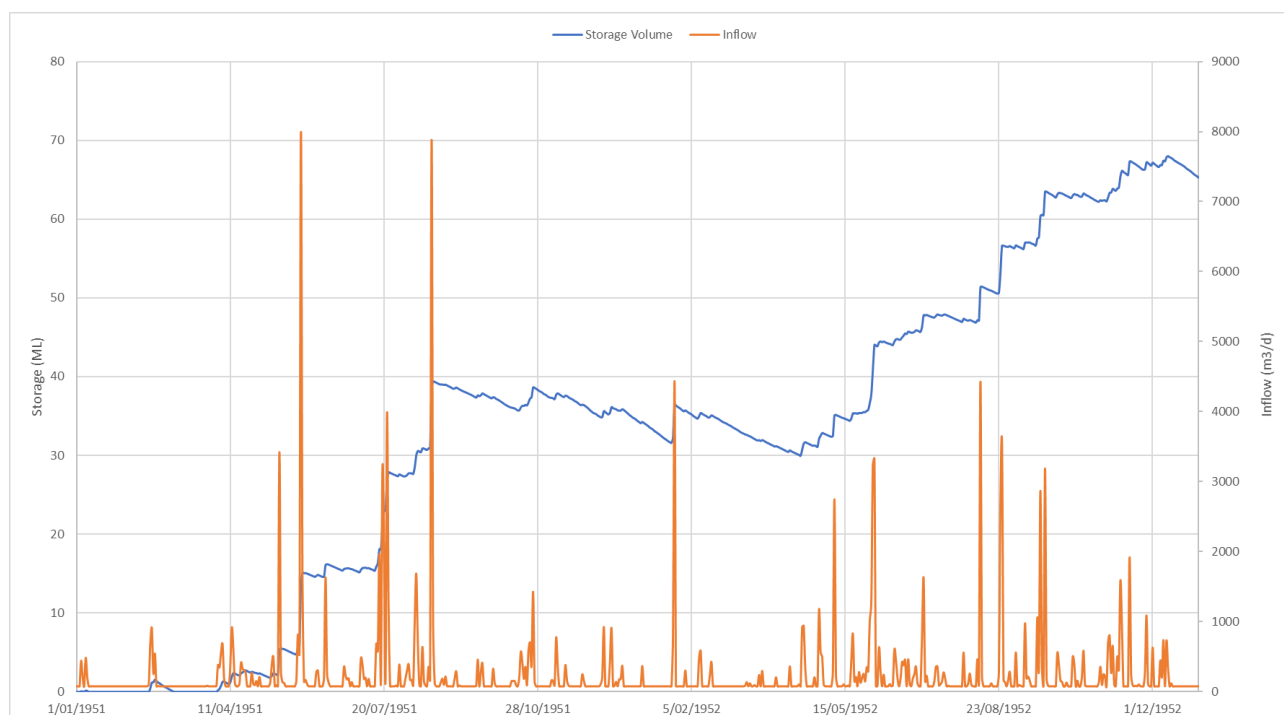
FIGURE 63 SCENARIO 2 – ADJUSTED 51/52 STORAGE VERSUS TIME
