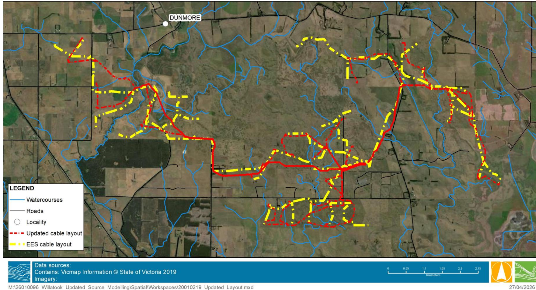
Figure A-3 Wind farm cable changes
