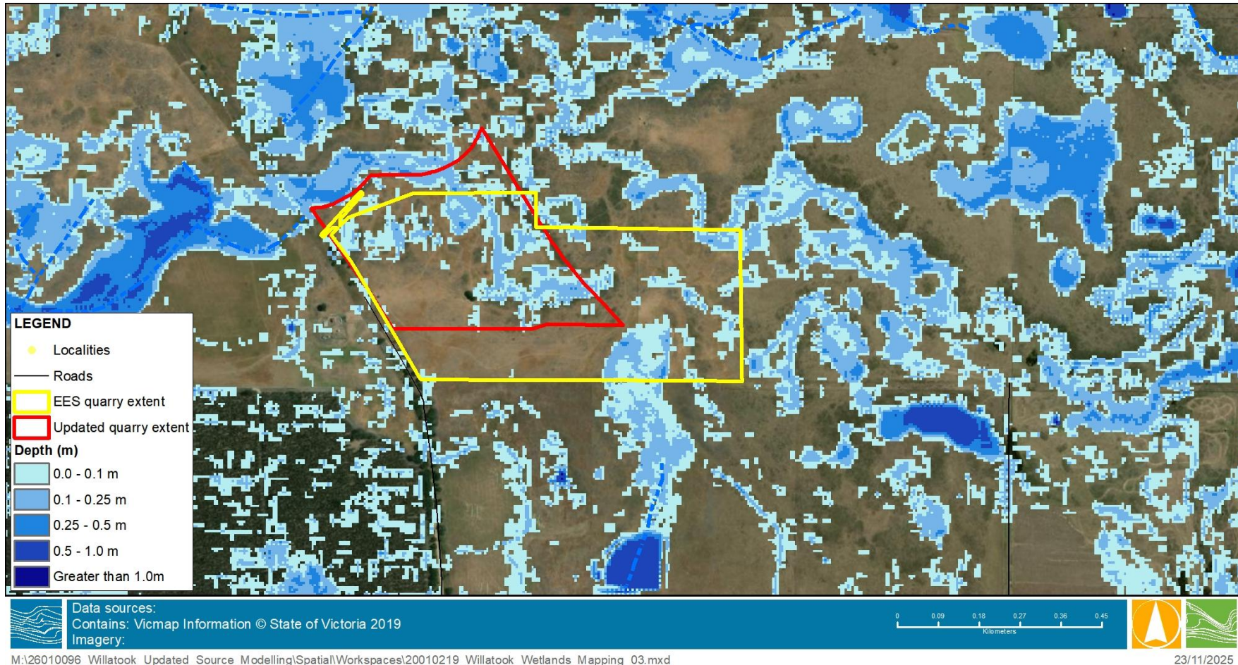
Figure 3-5 1% AEP depths within and surrounding the EES and updated quarry footprints.
