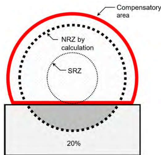
Figure 9. Sample (not to scale) of minor/moderate encroachment. AS4970:205, May 2025.
