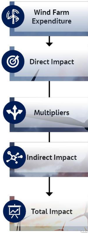
Figure 3: Input-output modelling
