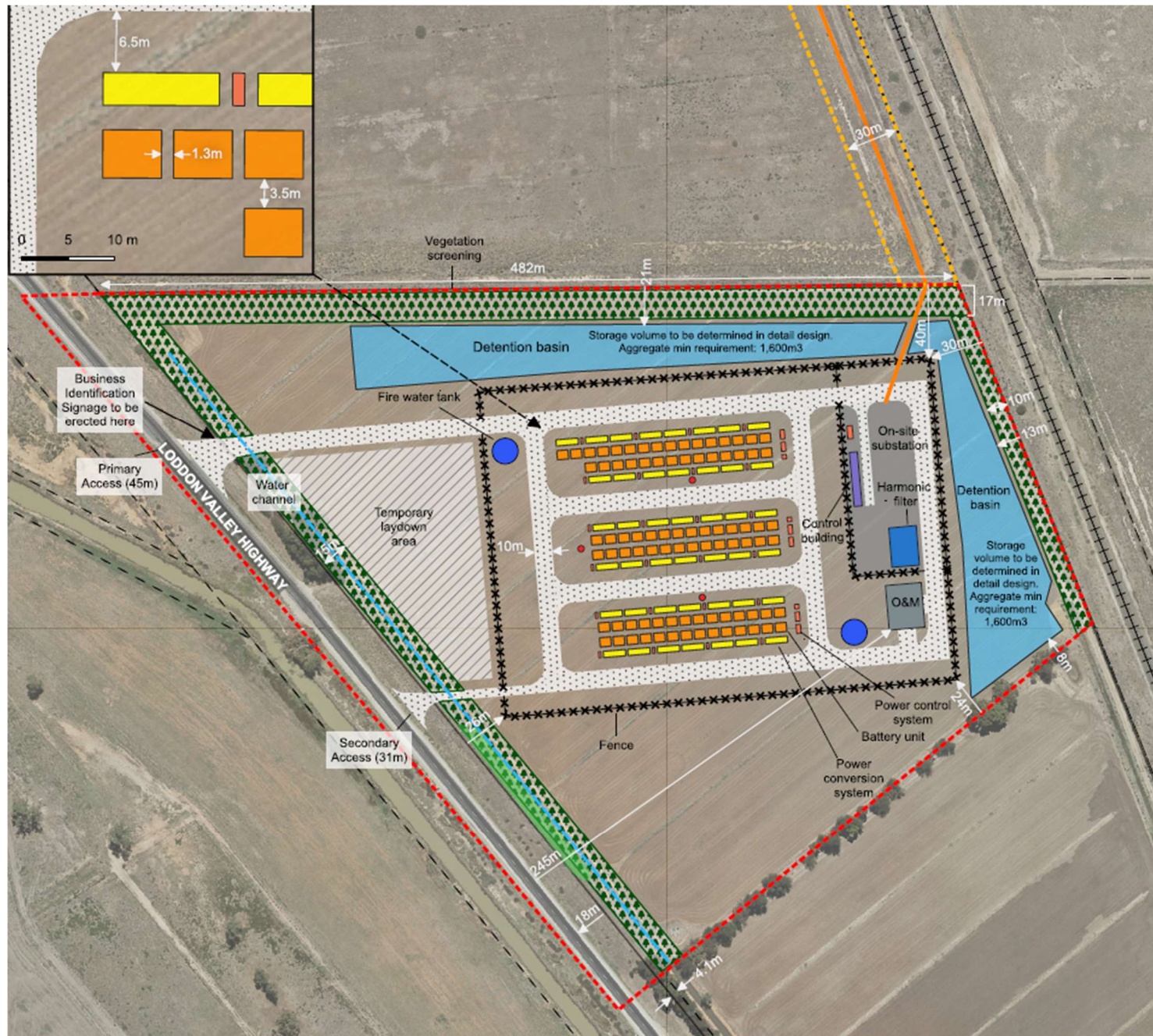
Figure 1 - Indicative Project Layout
