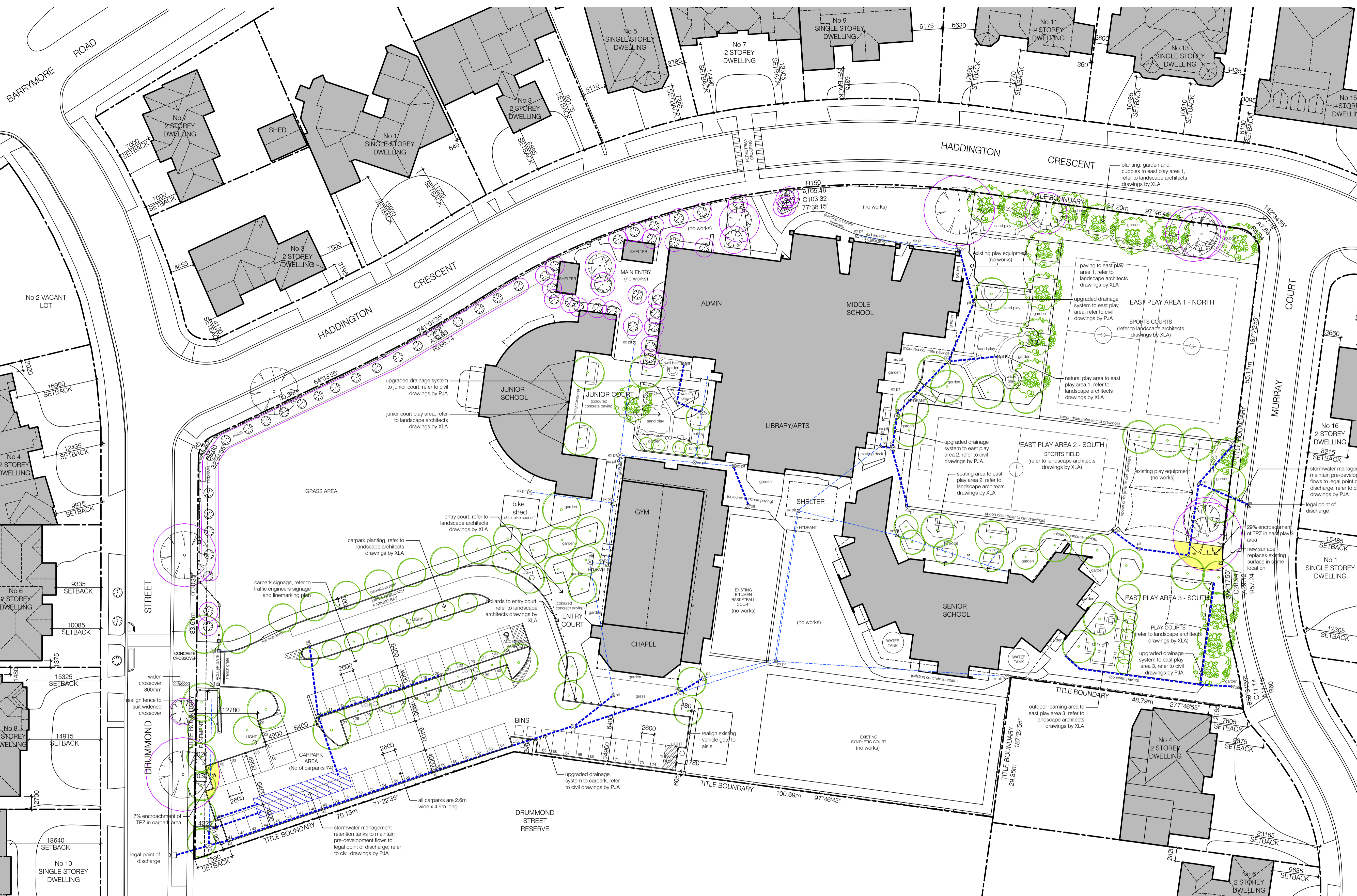
1 Proposed Site Plan REF: SCALE: 1:400 (A1)
