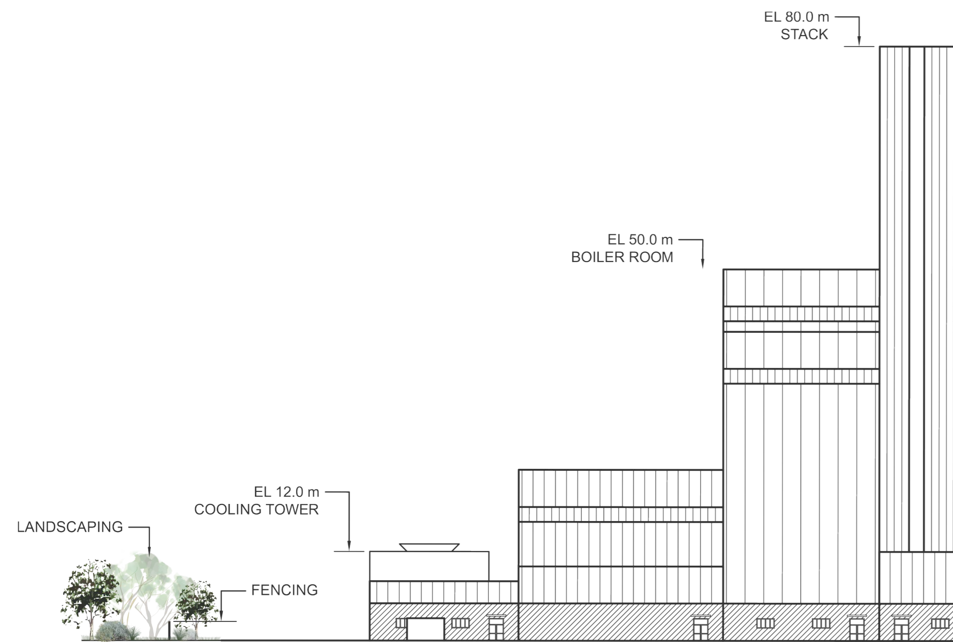
D2 Indicative Elevation 1:500 @ A1
