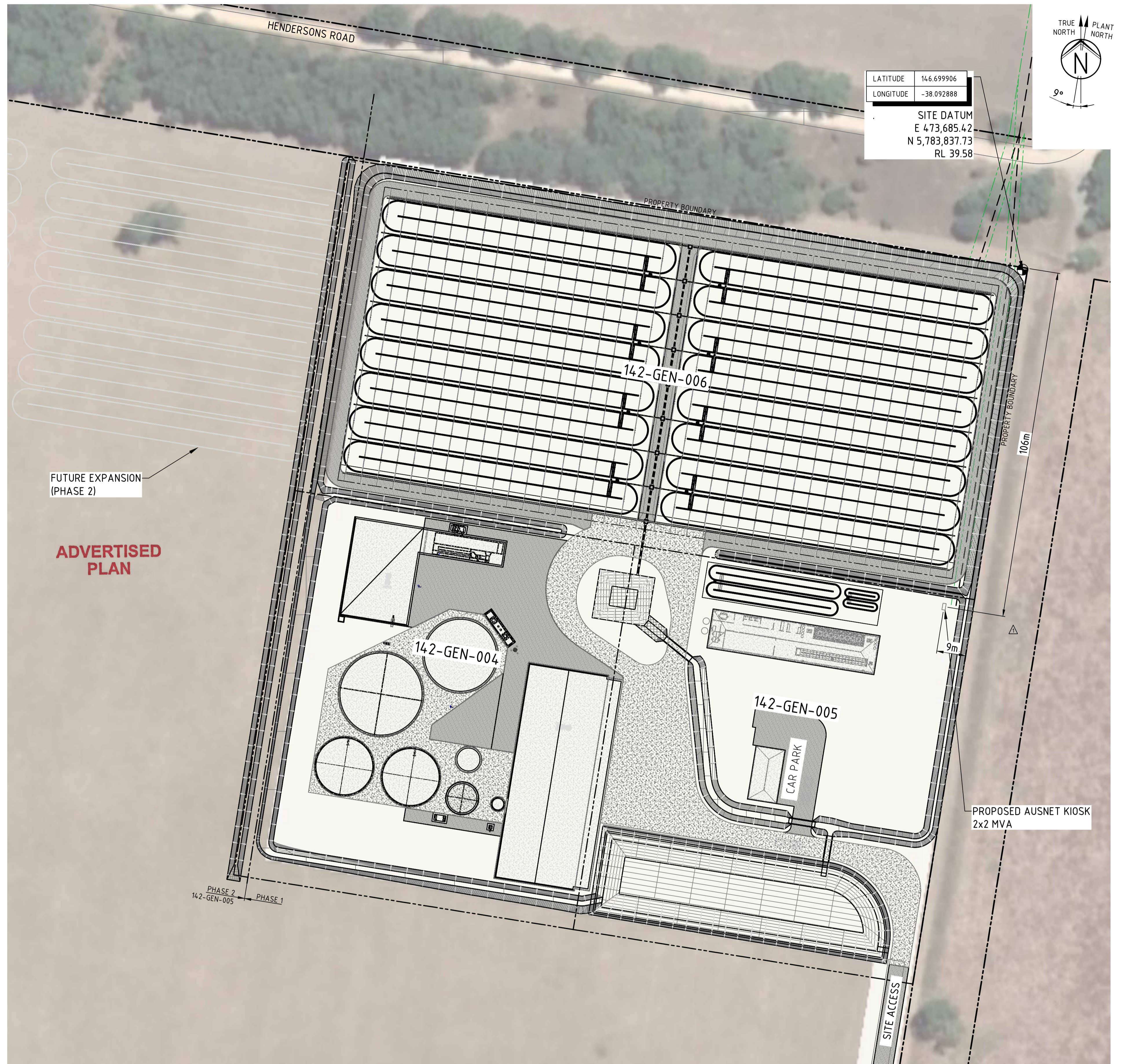
SITE LAYOUT & KEYPLAN SCALE NTS
