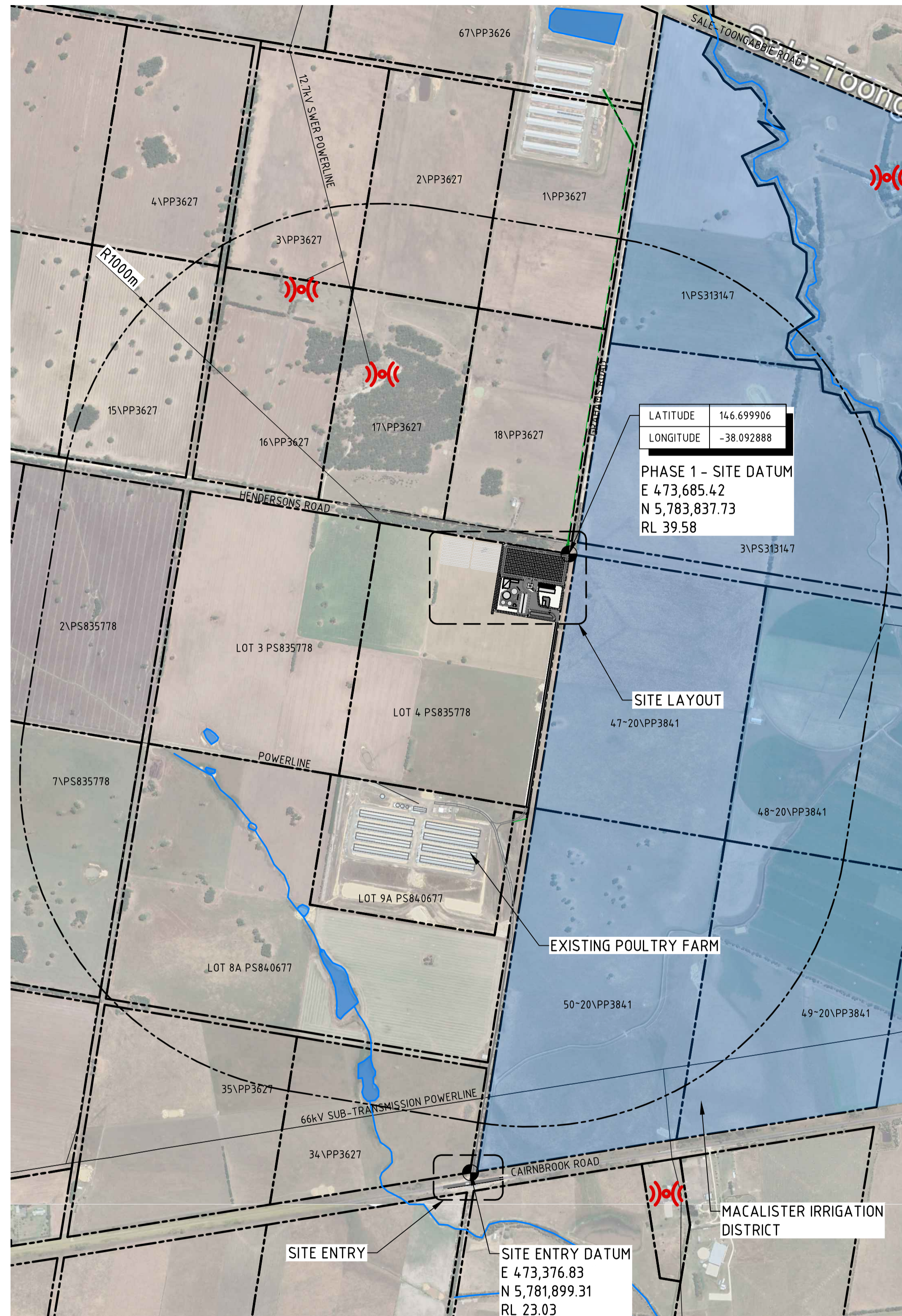
SITE CONTEXT SCALE 1:10,000
