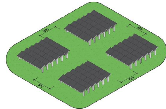
Figure 7: Six metre separation between solar panel banks (indicative only).
