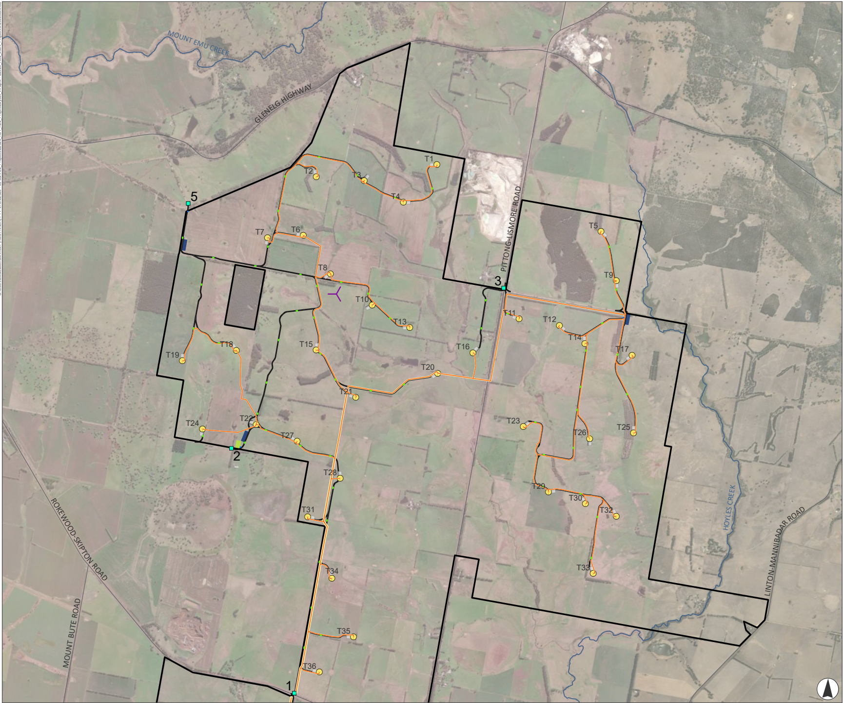
FIGURE 3.4a Project Infrastructure
