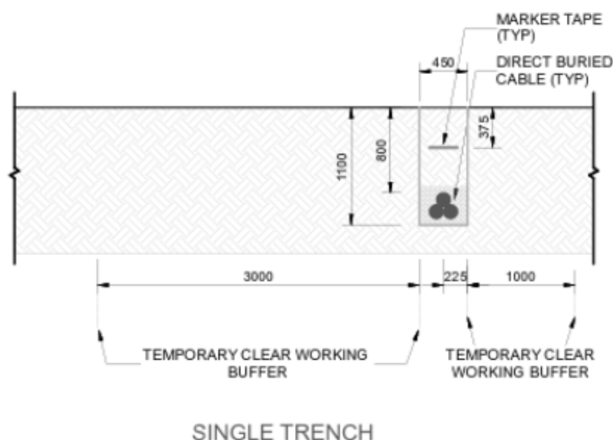
Photo 3.12 Indicative Single Cable Trench Design (measurements approximate and would be finalised in accordance with relevant standards and site conditions)
