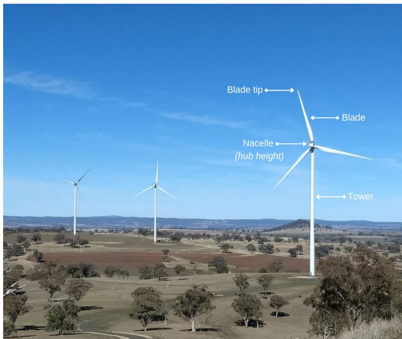
Photo 3.1 Components of a WTG as Shown at an existing Squadron Energy Wind Farm
