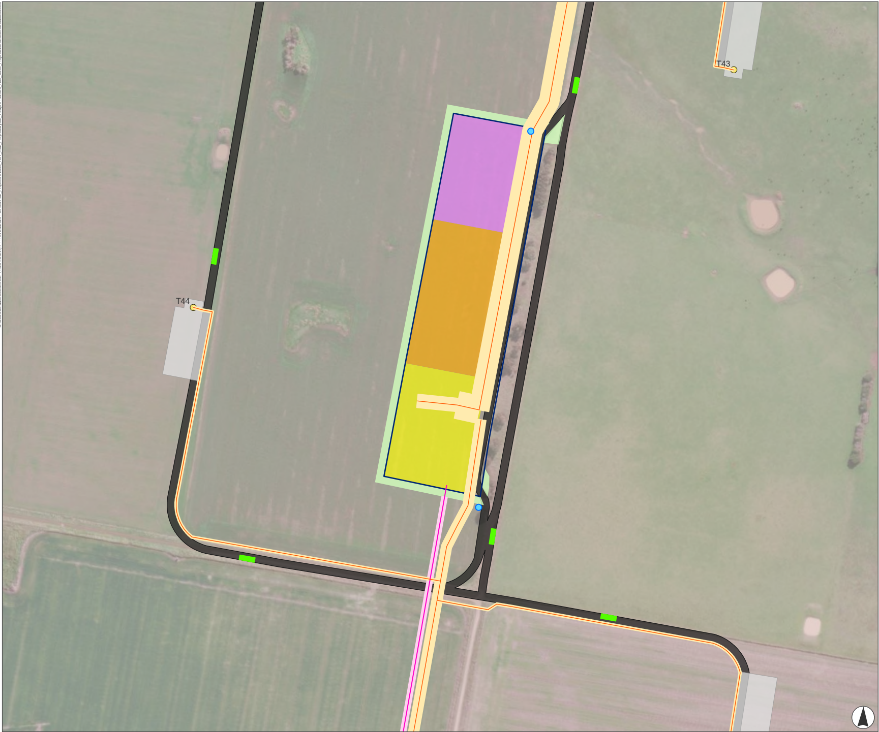
FIGURE 3.5 Project Infrastructure - Detailed BESS
