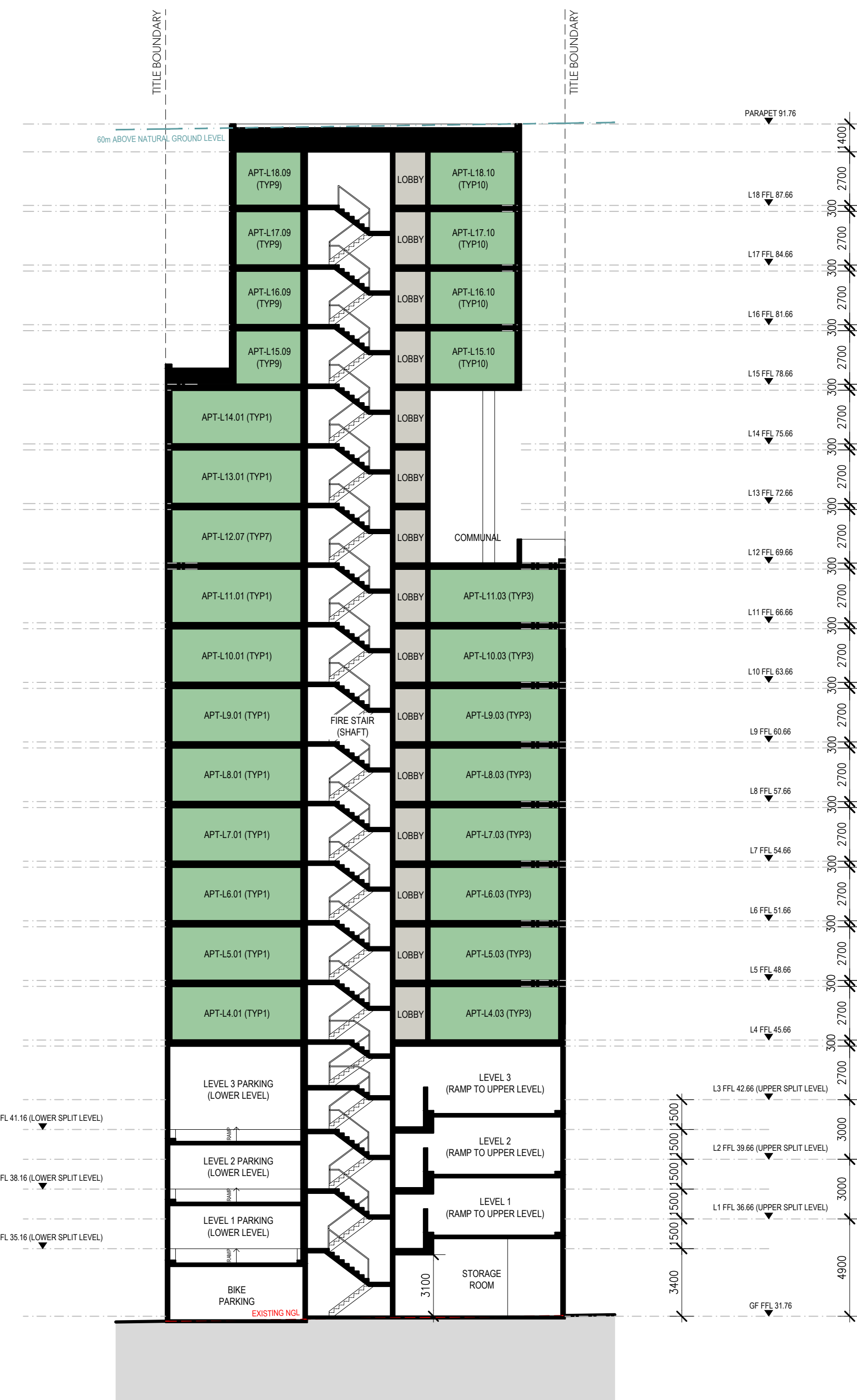
SECTION N B-B 1:200
