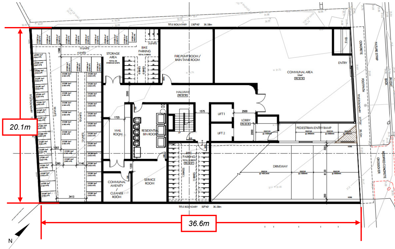
Figure 5: Ground floor plans with the plan-form dimensions overlaid.
