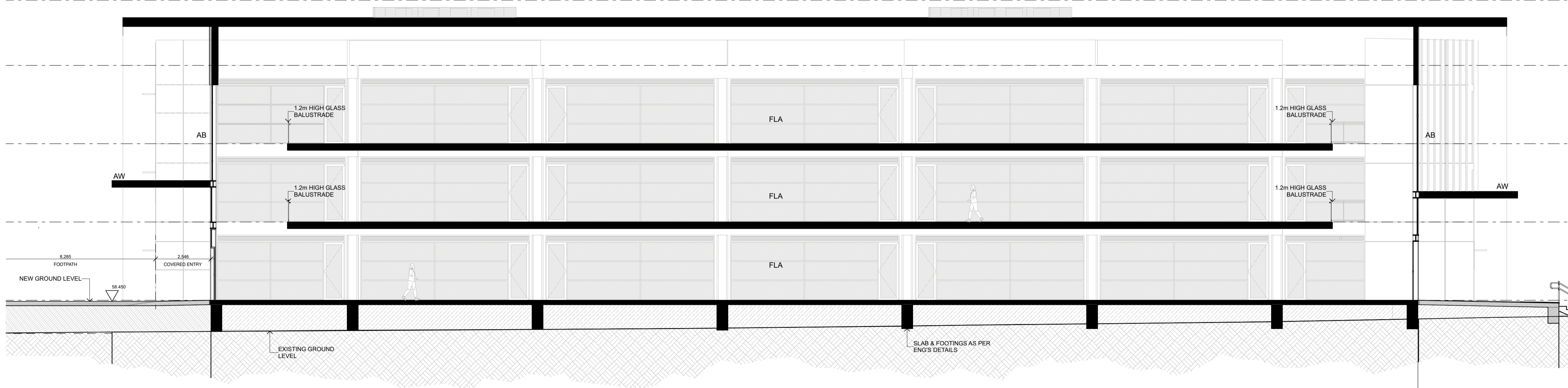
S-02 Section B Scale 1:100 (A3)
