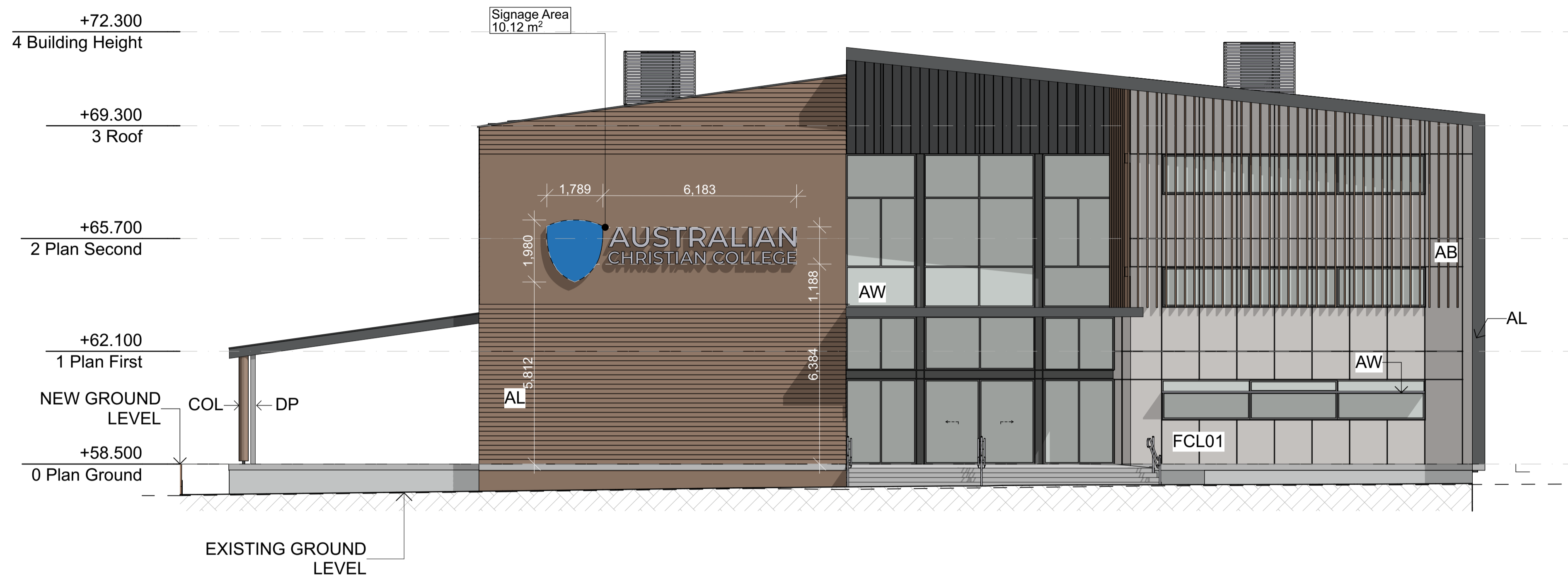
E-03 West Elevation - Proposed Signage Details WLayerID Scale 1:100
