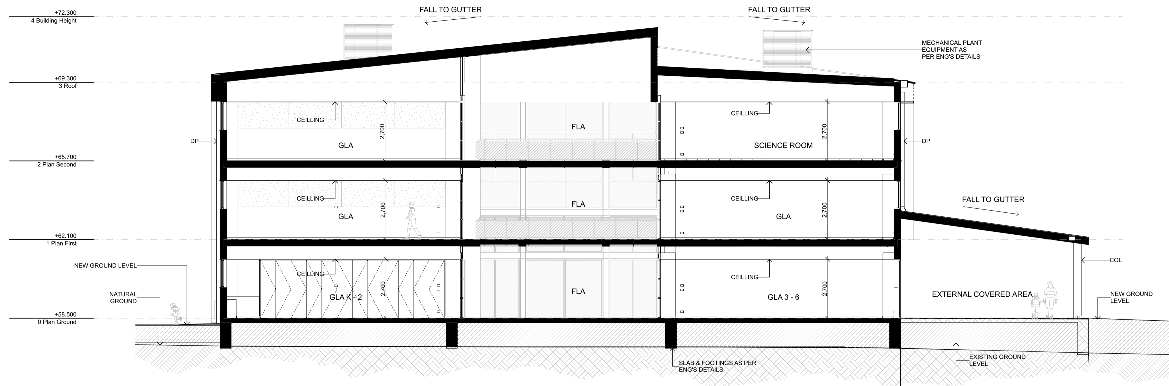
S-01 Section A Scale 1:100 (A3)
