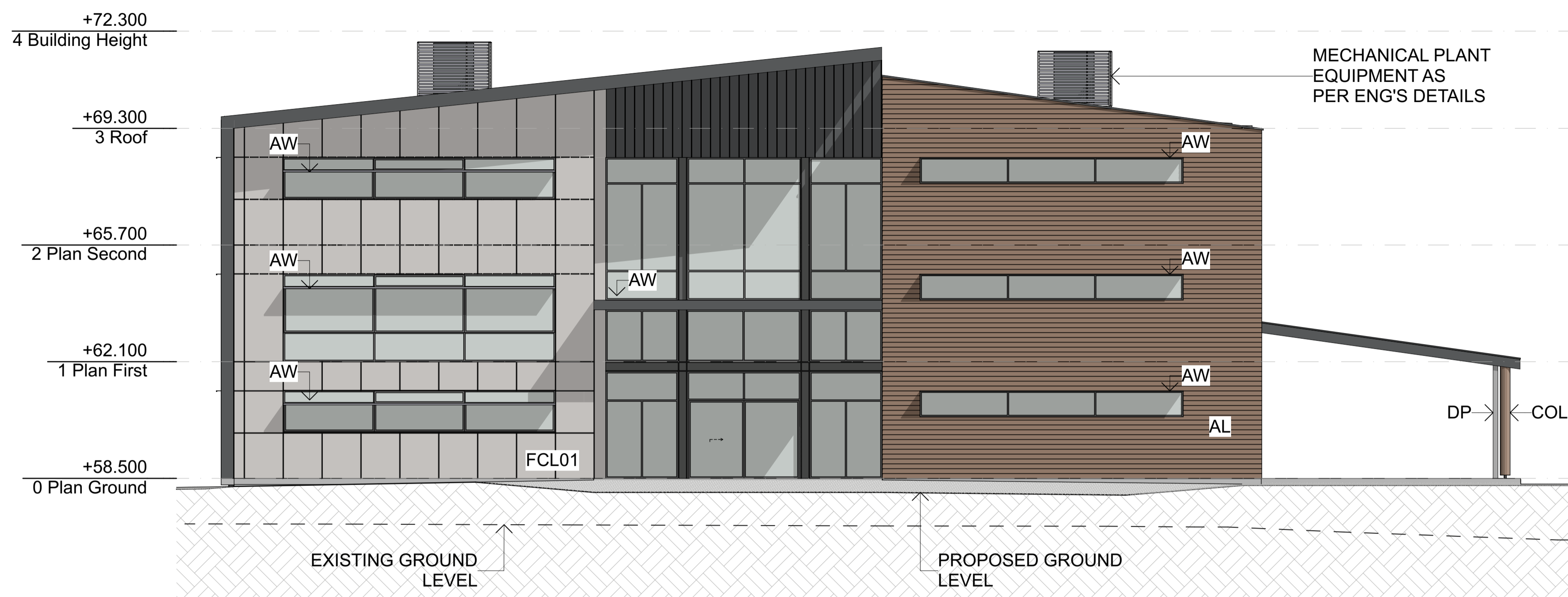
E-01 West Elevation Scale 1:100 (A3)
