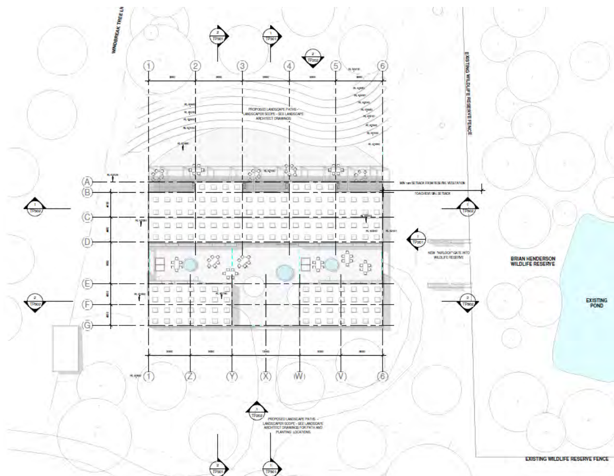
Figure 4. Excerpt from proposed Site Plan (Dwg. No. TP050, Rev. G). (McIldowie Partners, 5 September 2023).
