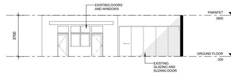
3 TP201 - EAST ELEVATION - COURTYARD
