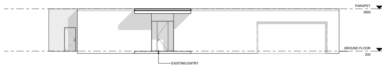
5 TP201 - EAST ELEVATION
