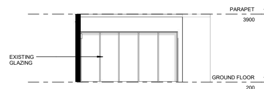
4 TP202 - WEST ELEVATION - COURTYARD
