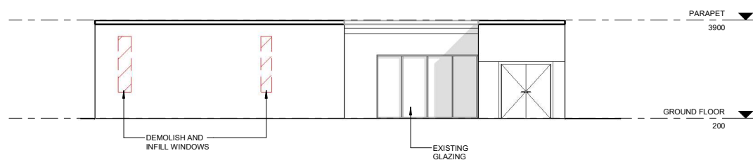
6 TP202 - WEST ELEVATION
