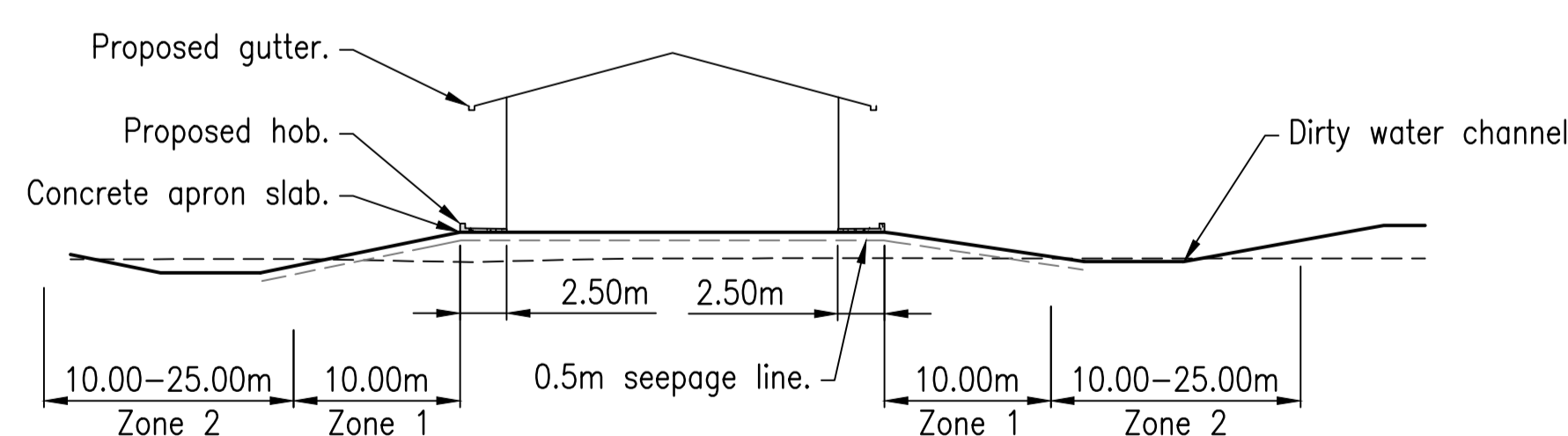
TYPICAL SHED SECTION Do not scale.
