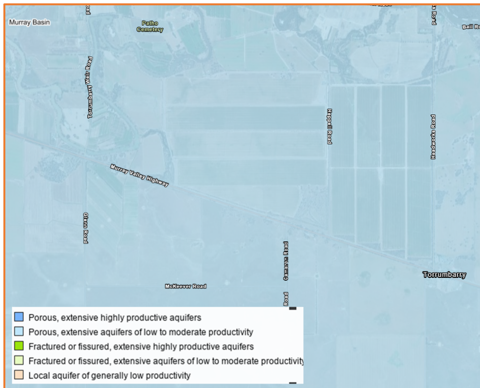
Figure 3-3: Groundwater Zoning Map (Geoscience Australia Portal).
