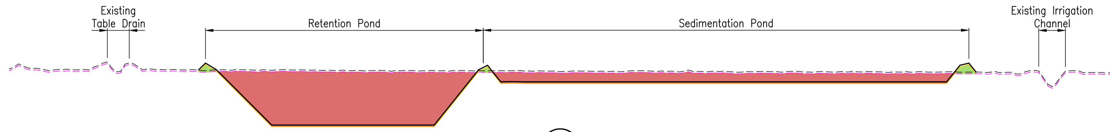
SECTION D SCALE 1:1000(H); 1:200(V) (A1) C-SK4004
