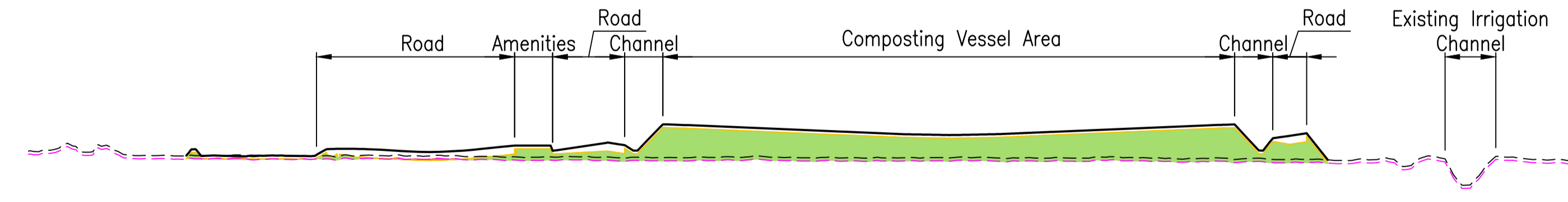
SECTION E SCALE 1:1000(H); 1:200(V) (A1) C-SK4004
