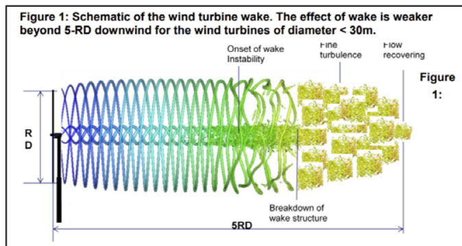
Figure 3: Schematic of WTG Wake (UK CAP 746- 2016)
